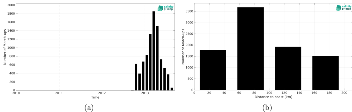
Figure 2: Number of match-ups between Surface drifters and Aquarius SSS L3 OR v5 - Monthly (NASA-GSFC) SSS as a function of time (a) and as function of the distance to coast (b) over the Mediterranean Sea Pi-MEP region and for the full satellite product period.
