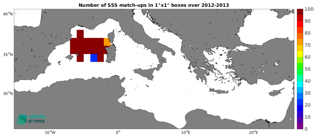
Figure 4: Number of SSS match-ups between Surface drifters SSS and the Aquarius SSS L3 OR v5 - Monthly (NASA-GSFC) SSS product for the Mediterranean Sea Pi-MEP region over 1^\circ \times 1^\circ boxes and for the full satellite product period.
