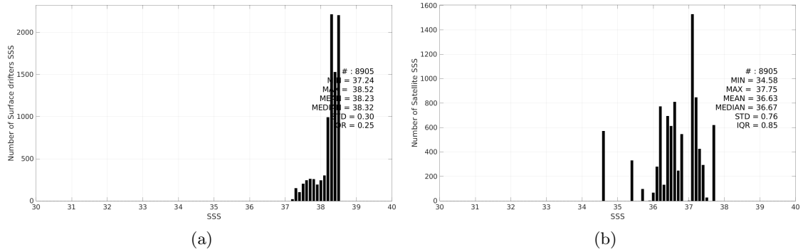
Figure 3: Histograms of SSS from Surface drifters (a) and Aquarius SSS L3 OR v5 - Monthly (NASA-GSFC) (b) considering all match-up pairs per bins of 0.1 over the Mediterranean Sea Pi-MEP region and for the full satellite product period.
