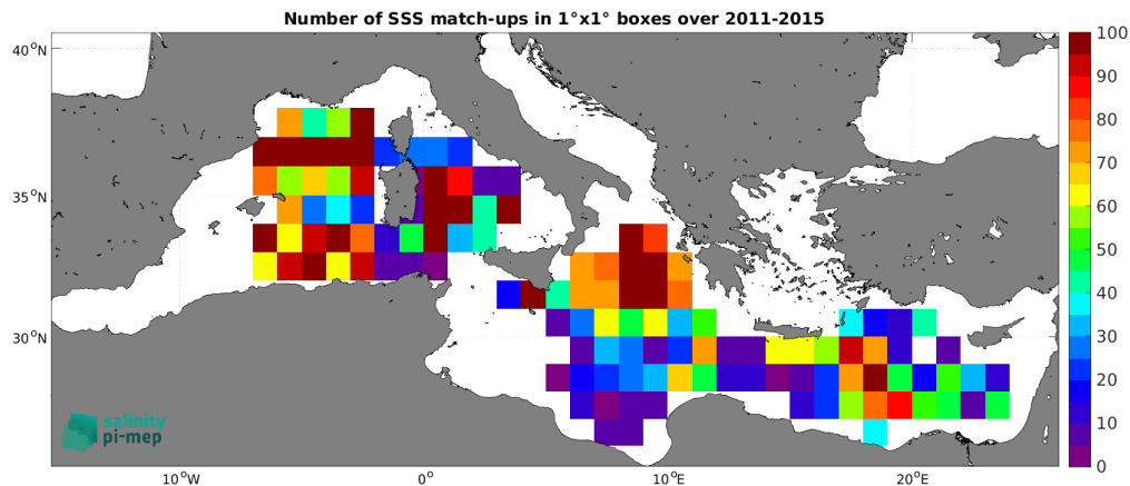
Figure 4: Number of SSS match-ups between Argo SSS and the Aquarius SSS L3 OR v5 - Monthly (NASA-GSFC) SSS product for the Mediterranean Sea Pi-MEP region over 1^\circ \times 1^\circ boxes and for the full satellite product period.
