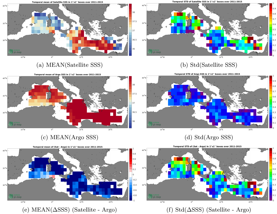
Figure 6: Temporal mean (left) and Std (right) of SSS from Aquarius SSS L3 OR v5 - Monthly (NASA-GSFC) (top), Argo (middle), and of \Delta\text{SSS} (Satellite - Argo). Only match-up pairs are used to generate these maps.
