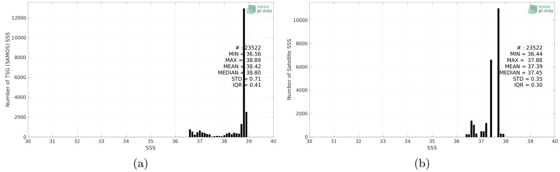
Figure 2: Histograms of SSS from TSG (SAMOS) (a) and Aquarius SSS L3 OR v5 - Monthly - Rain mask (NASA-GSFC) (b) considering all match-up pairs per bins of 0.1 over the Mediterranean Sea Pi-MEP region and for the full satellite product period.
