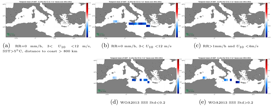
Figure 12: Temporal mean gridded over spatial boxes of size 1^{\circ}\times 1^{\circ} of \Delta\text{SSS} (Aquarius SSS L3 OR v5 - Monthly - Rain mask (NASA-GSFC) - TSG (SAMOS)) for 5 different subdatasets corresponding to:RR=0 mm/h, 3 < U_{10} < 12 m/s, SST > 5^{\circ}\text{C} , distance to coast > 800 km (a), RR=0 mm/h, 3 < U_{10} < 12 m/s (b), RR > 1 mm/h and U_{10} < 4 m/s (c), WOA2013 SSS Std < 0.2 (d), WOA2013 SSS Std > 0.2 (e).
