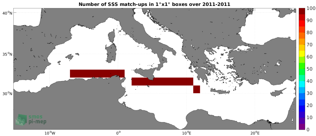
Figure 4: Number of SSS match-ups between TSG (SAMOS) SSS and the Aquarius SSS L3 OR v5 - Monthly - Rain mask (NASA-GSFC) SSS product for the Mediterranean Sea Pi-MEP region over 1^\circ \times 1^\circ boxes and for the full satellite product period.
