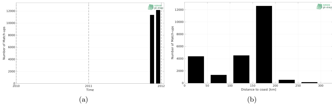
Figure 1: Number of match-ups between TSG (SAMOS) and Aquarius SSS L3 OR v5 - Monthly - Rain mask (NASA-GSFC) SSS as a function of time (a) and as function of the distance to coast (b) over the Mediterranean Sea Pi-MEP region and for the full satellite product period.
