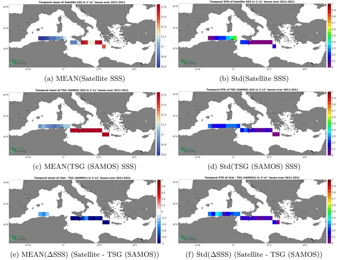
Figure 6: Temporal mean (left) and Std (right) of SSS from Aquarius SSS L3 OR v5 - Monthly - Rain mask (NASA-GSFC) (top), TSG (SAMOS) (middle), and of \Delta\text{SSS} (Satellite - TSG (SAMOS)). Only match-up pairs are used to generate these maps.
