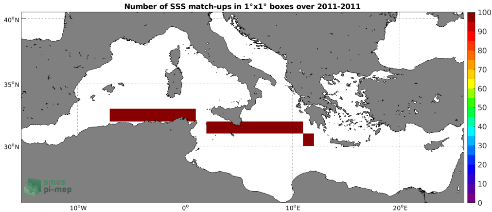
Figure 4: Number of SSS match-ups between TSG (SAMOS) SSS and the Aquarius SSS L3 OR v5 - Monthly - Rain mask (NASA-GSFC) SSS product for the Mediterranean Sea Pi-MEP region over 1°x1° boxes and for the full satellite product period.
