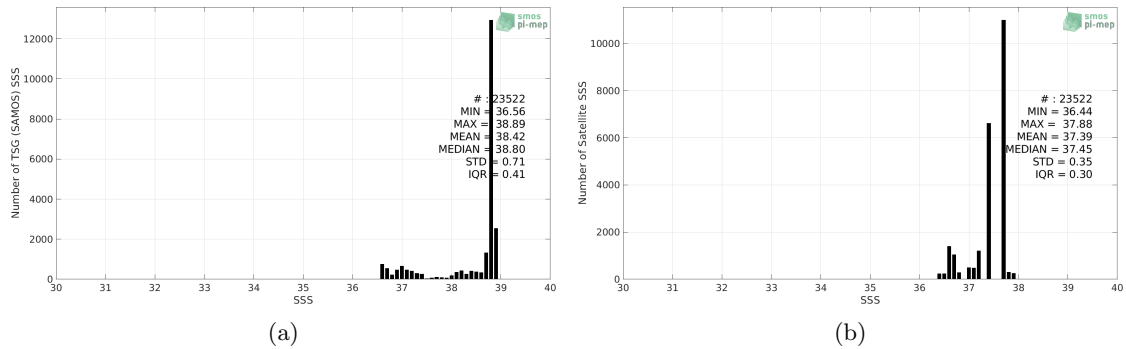
Figure 2: Histograms of SSS from TSG (SAMOS) (a) and Aquarius SSS L3 OR v5 - Monthly - Rain mask (NASA-GSFC) (b) considering all match-up pairs per bins of 0.1 over the Mediterranean Sea Pi-MEP region and for the full satellite product period.
