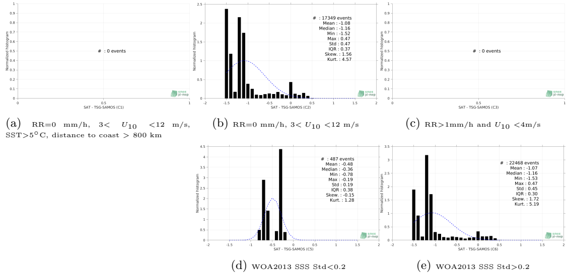
Figure 13: Normalized histogram of \Delta SSS (Aquarius-L3-OR-V5-MONTHLY-RAIN-MASK-1DEG - TSG-SAMOS) for 5 different subdatasets corresponding to: RR=0 mm/h, 3 < U_{10} < 12 m/s, SST>5°C, distance to coast > 800 km (a), RR=0 mm/h, 3 < U_{10} < 12 m/s (b), RR>1mm/h and U_{10} < 4 m/s (c), WOA2013 SSS Std<0.2 (d), WOA2013 SSS Std>0.2 (e).
