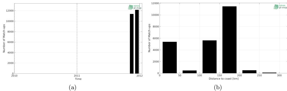
Figure 1: Number of match-ups between TSG-SAMOS and Aquarius-L3-OR-V5-MONTHLY-RAIN-MASK-1DEG SSS as a function of time (a) and as function of the distance to coast (b) over the Mediterranean Sea Pi-MEP region and for the full satellite product period.
