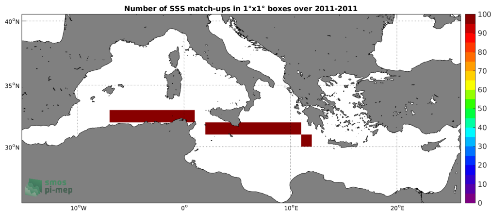
Figure 4: Number of SSS match-ups between TSG-SAMOS SSS and the Aquarius-L3-OR-V5-MONTHLY-RAIN-MASK-1DEG SSS product for the Mediterranean Sea Pi-MEP region over 1^\circ \times 1^\circ boxes and for the full satellite product period.
