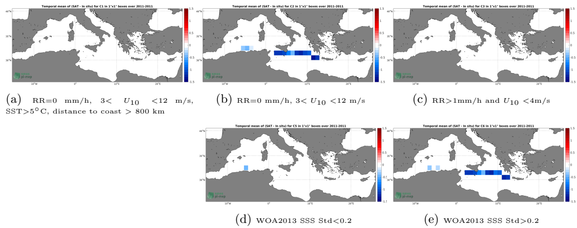
Figure 12: Temporal mean gridded over spatial boxes of size 1^\circ \times 1^\circ of \Delta SSS (Aquarius-L3-OR-V5-MONTHLY-RAIN-MASK-1DEG - TSG-SAMOS) for 5 different subdatasets corresponding to:RR=0 mm/h, 3 < U_{10} < 12 m/s, SST >5^\circ C, distance to coast > 800 km (a), RR=0 mm/h, 3 < U_{10} < 12 m/s (b), RR >1 mm/h and U_{10} < 4 m/s (c), WOA2013 SSS Std <0.2 (d), WOA2013 SSS Std >0.2 (e).
