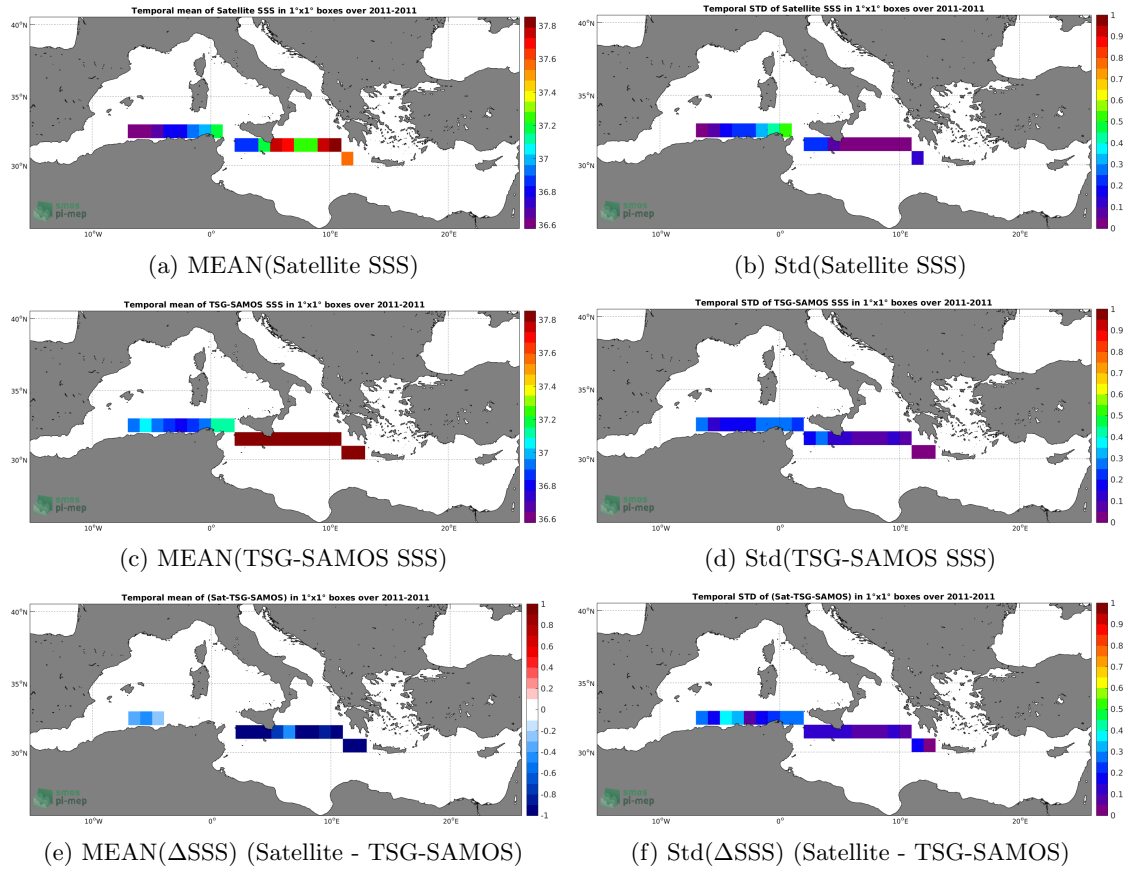
Figure 6: Temporal mean (left) and Std (right) of SSS from Aquarius-L3-OR-V5-MONTHLY-RAIN-MASK-1DEG (top), TSG-SAMOS (middle), and of \Delta SSS (Satellite - TSG-SAMOS). Only match-up pairs are used to generate these maps.
