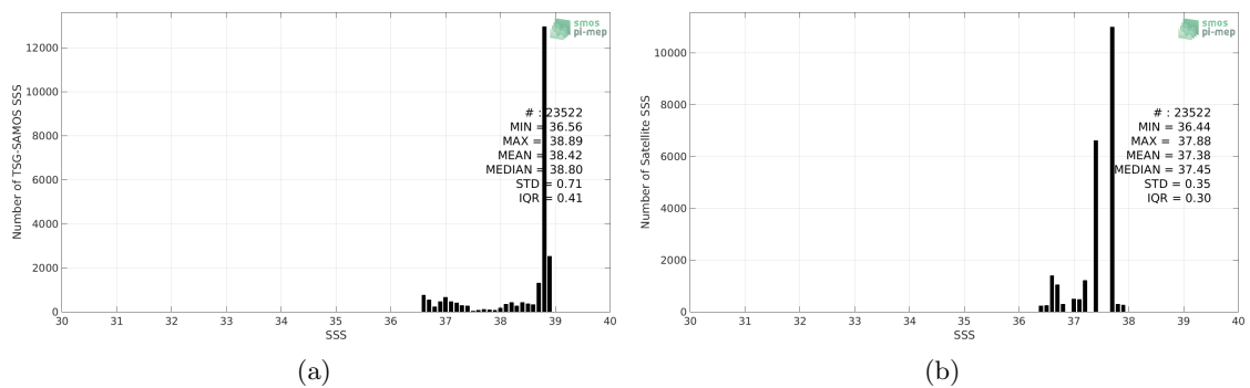
Figure 2: Histograms of SSS from TSG-SAMOS (a) and Aquarius-L3-OR-V5-MONTHLY-RAIN-MASK-1DEG (b) considering all match-up pairs per bins of 0.1 over the Mediterranean Sea Pi-MEP region and for the full satellite product period.
