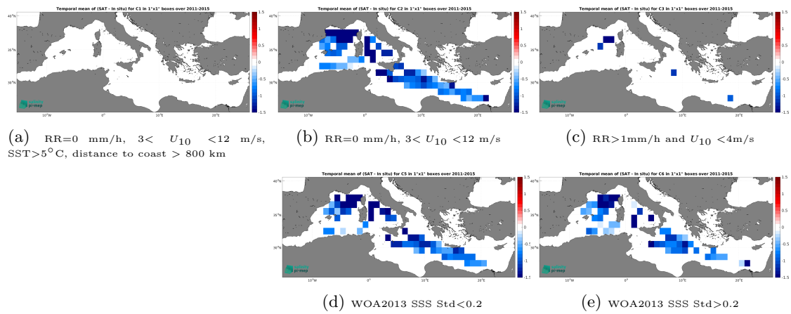
Figure 14: Temporal mean gridded over spatial boxes of size 1^\circ \times 1^\circ of \Delta SSS (Aquarius SSS L3 OR v5 - Monthly - Rain mask (NASA-GSFC) - TSG (LEGOS-DM)) for 5 different subdatasets corresponding to:RR=0 mm/h, 3 < U_{10} < 12 m/s, SST >5^\circ\text{C} , distance to coast > 800 km (a), RR=0 mm/h, 3 < U_{10} < 12 m/s (b), RR >1 mm/h and U_{10} < 4 m/s (c), WOA2013 SSS Std <0.2 (d), WOA2013 SSS Std >0.2 (e).
