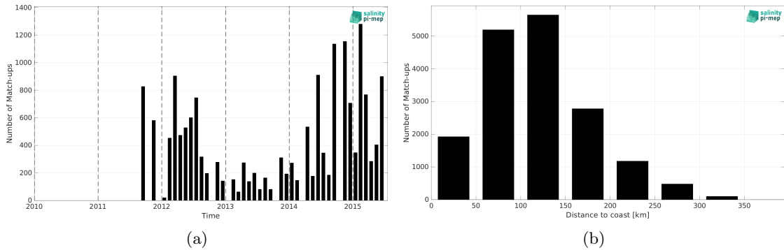
Figure 2: Number of match-ups between TSG (LEGOS-DM) and Aquarius SSS L3 OR v5 - Monthly - Rain mask (NASA-GSFC) SSS as a function of time (a) and as function of the distance to coast (b) over the Mediterranean Sea Pi-MEP region and for the full satellite product period.
