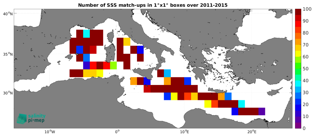
Figure 5: Number of SSS match-ups between TSG (LEGOS-DM) SSS and the Aquarius SSS L3 OR v5 - Monthly - Rain mask (NASA-GSFC) SSS product for the Mediterranean Sea Pi-MEP region over 1^\circ \times 1^\circ boxes and for the full satellite product period.
