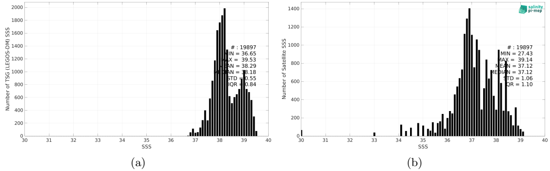
Figure 2: Histograms of SSS from TSG (LEGOS-DM) (a) and Aquarius SSS L3 OR v5 - Monthly - Rain mask (NASA-GSFC) (b) considering all match-up pairs per bins of 0.1 over the Mediterranean Sea Pi-MEP region and for the full satellite product period.
