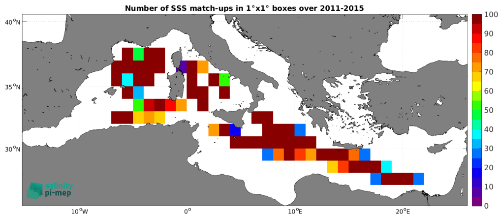
Figure 4: Number of SSS match-ups between TSG (LEGOS-DM) SSS and the Aquarius SSS L3 OR v5 - Monthly - Rain mask (NASA-GSFC) SSS product for the Mediterranean Sea Pi-MEP region over 1^\circ \times 1^\circ boxes and for the full satellite product period.
