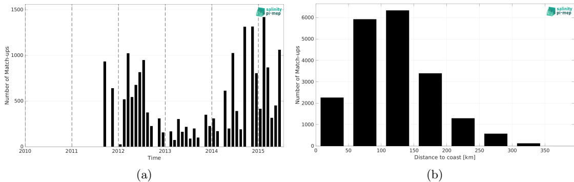
Figure 1: Number of match-ups between TSG (LEGOS-DM) and Aquarius SSS L3 OR v5 - Monthly - Rain mask (NASA-GSFC) SSS as a function of time (a) and as function of the distance to coast (b) over the Mediterranean Sea Pi-MEP region and for the full satellite product period.
