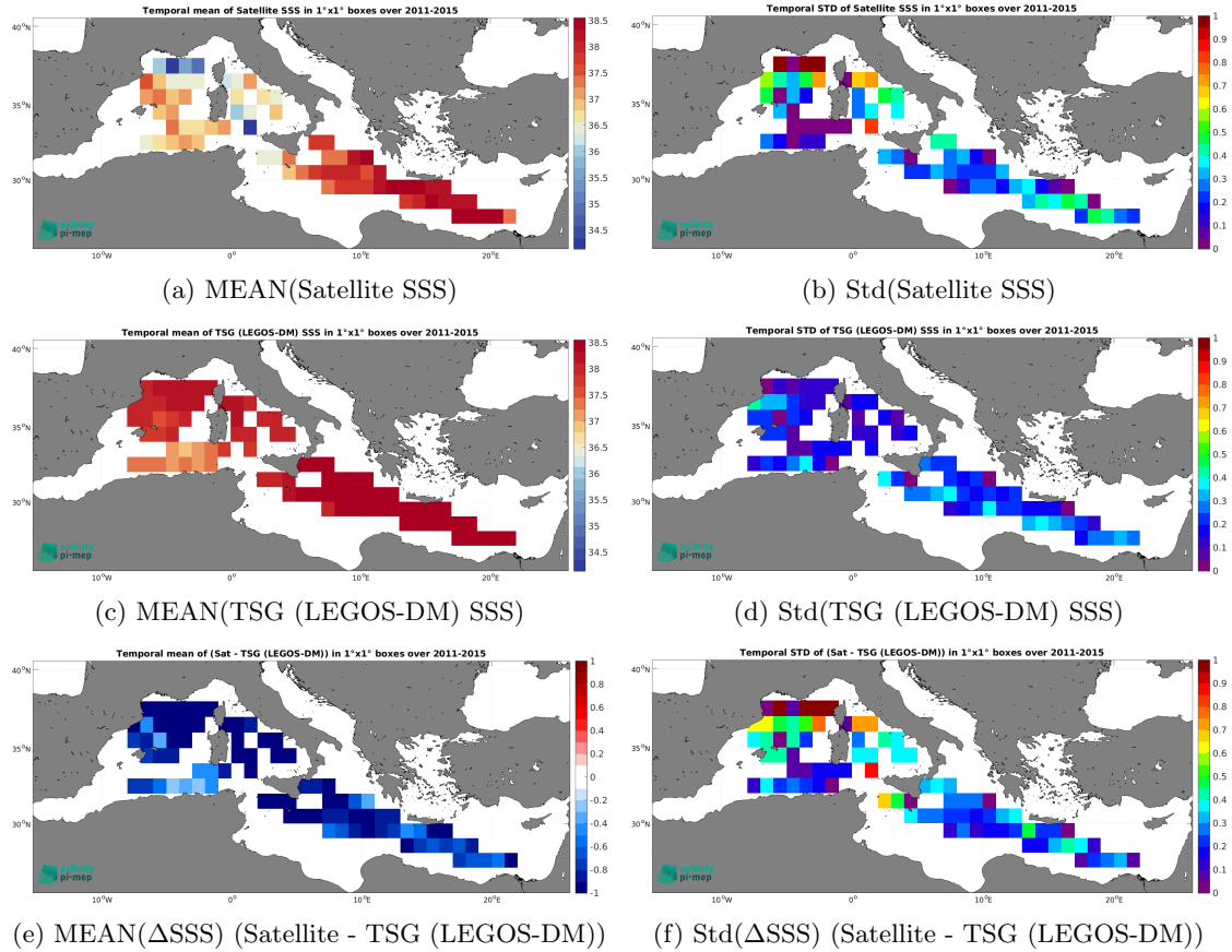
Figure 6: Temporal mean (left) and Std (right) of SSS from Aquarius SSS L3 OR v5 - Monthly - Rain mask (NASA-GSFC) (top), TSG (LEGOS-DM) (middle), and of \Delta\text{SSS} (Satellite - TSG (LEGOS-DM)). Only match-up pairs are used to generate these maps.
