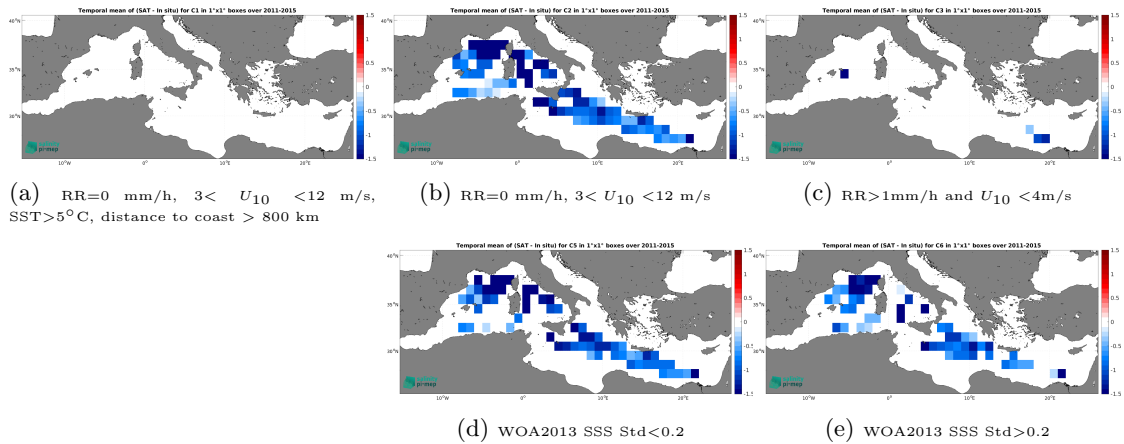
Figure 12: Temporal mean gridded over spatial boxes of size 1^{\circ}\times 1^{\circ} of \Delta\text{SSS} (Aquarius SSS L3 OR v5 - Monthly - Rain mask (NASA-GSFC) - TSG (LEGOS-DM)) for 5 different subdatasets corresponding to:RR=0 mm/h, 3 < U_{10} < 12 m/s, SST >5^{\circ}\text{C} , distance to coast > 800 km (a), RR=0 mm/h, 3 < U_{10} < 12 m/s (b), RR >1 mm/h and U_{10} < 4 m/s (c), WOA2013 SSS Std <0.2 (d), WOA2013 SSS Std >0.2 (e).
