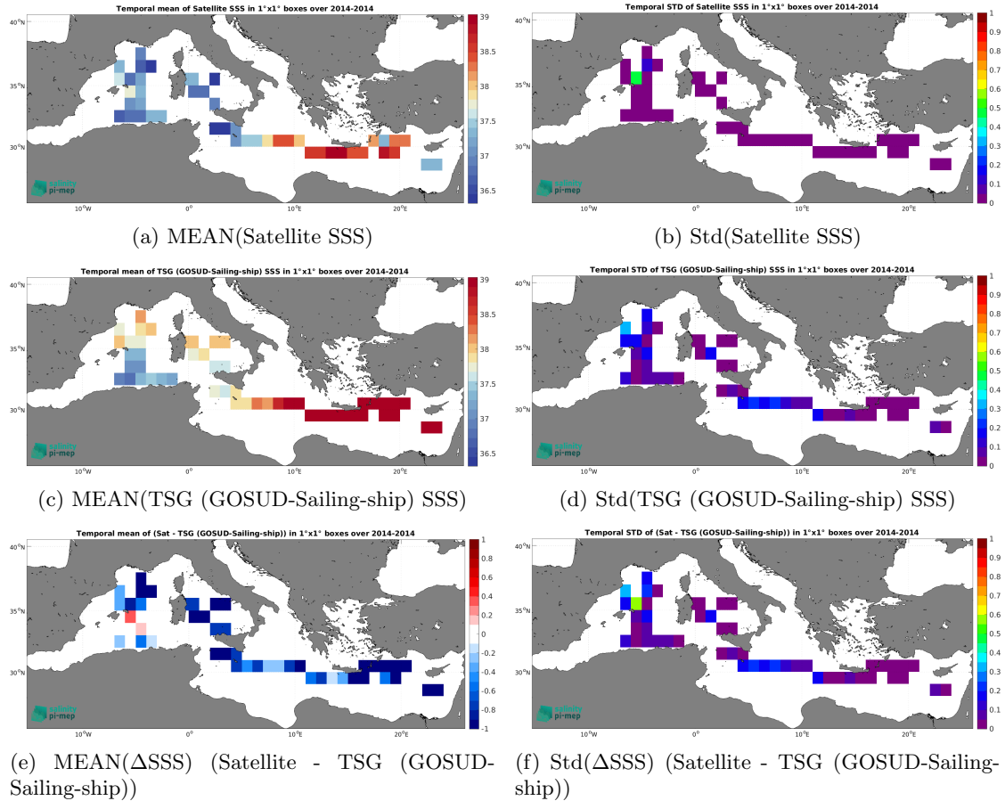
Figure 7: Temporal mean (left) and Std (right) of SSS from Aquarius SSS L3 OR v5 - Monthly - Rain mask (NASA-GSFC) (top), TSG (GOSUD-Sailing-ship) (middle), and of \Delta\text{SSS} (Satellite - TSG (GOSUD-Sailing-ship)). Only match-up pairs are used to generate these maps.
