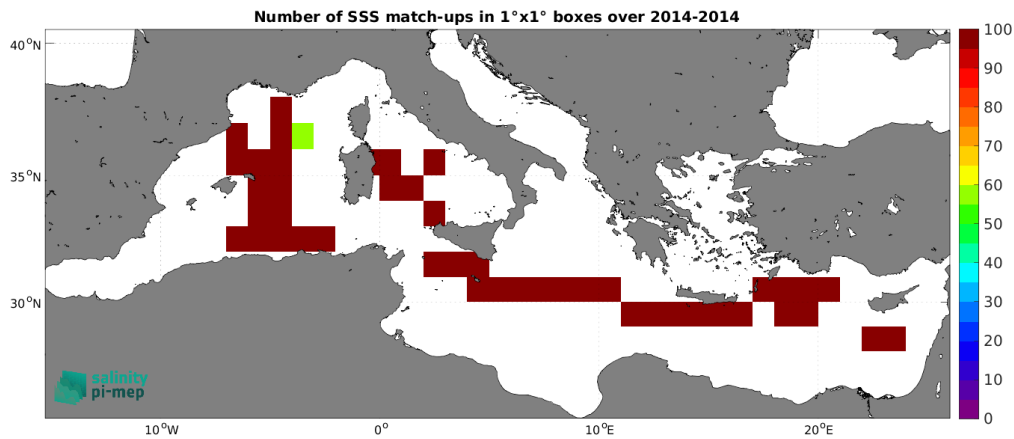
Figure 5: Number of SSS match-ups between TSG (GOSUD-Sailing-ship) SSS and the Aquarius SSS L3 OR v5 - Monthly - Rain mask (NASA-GSFC) SSS product for the Mediterranean Sea Pi-MEP region over 1^\circ \times 1^\circ boxes and for the full satellite product period.
