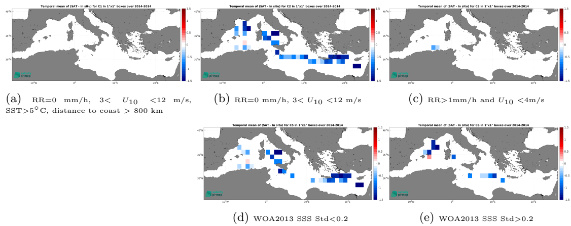
Figure 14: Temporal mean gridded over spatial boxes of size 1^\circ \times 1^\circ of \Delta SSS (Aquarius SSS L3 OR v5 - Monthly - Rain mask (NASA-GSFC) - TSG (GOSUD-Sailing-ship)) for 5 different subdatasets corresponding to:RR=0 mm/h, 3 < U_{10} < 12 m/s, SST >5^\circ\text{C} , distance to coast > 800 km (a), RR=0 mm/h, 3 < U_{10} < 12 m/s (b), RR >1 mm/h and U_{10} < 4 m/s (c), WOA2013 SSS Std <0.2 (d), WOA2013 SSS Std >0.2 (e).
