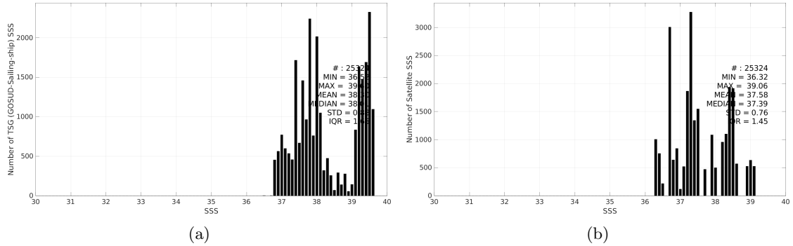
Figure 3: Histograms of SSS from TSG (GOSUD-Sailing-ship) (a) and Aquarius SSS L3 OR v5 - Monthly - Rain mask (NASA-GSFC) (b) considering all match-up pairs per bins of 0.1 over the Mediterranean Sea Pi-MEP region and for the full satellite product period.
