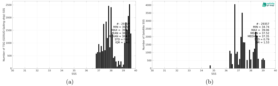
Figure 2: Histograms of SSS from TSG (GOSUD-Sailing-ship) (a) and Aquarius SSS L3 OR v5 - Monthly - Rain mask (NASA-GSFC) (b) considering all match-up pairs per bins of 0.1 over the Mediterranean Sea Pi-MEP region and for the full satellite product period.
