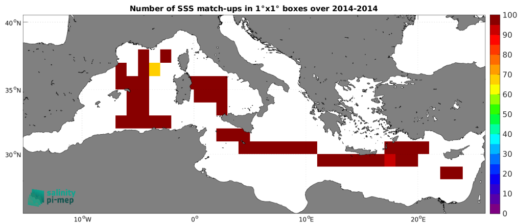
Figure 4: Number of SSS match-ups between TSG (GOSUD-Sailing-ship) SSS and the Aquarius SSS L3 OR v5 - Monthly - Rain mask (NASA-GSFC) SSS product for the Mediterranean Sea Pi-MEP region over 1^\circ \times 1^\circ boxes and for the full satellite product period.
