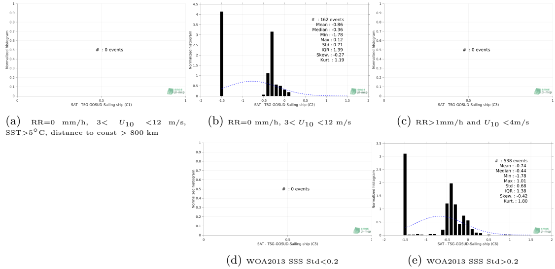
Figure 13: Normalized histogram of \Delta SSS (Aquarius-L3-OR-V5-MONTHLY-RAIN-MASK-1DEG - TSG-GOSUD-Sailing-ship) for 5 different subdatasets corresponding to: RR=0 mm/h, 3 < U_{10} < 12 m/s, SST > 5°C, distance to coast > 800 km (a), RR=0 mm/h, 3 < U_{10} < 12 m/s (b), RR > 1mm/h and U_{10} < 4 m/s (c), WOA2013 SSS Std < 0.2 (d), WOA2013 SSS Std > 0.2 (e).
