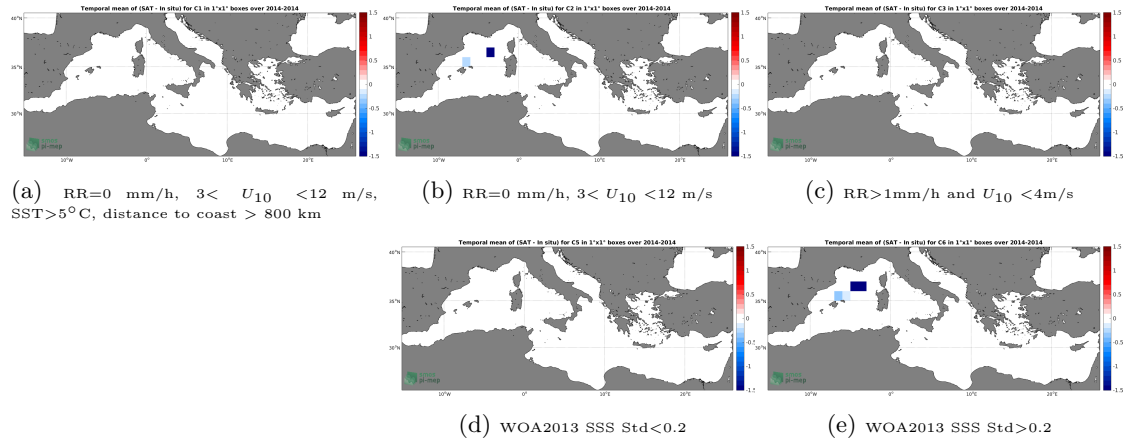
Figure 12: Temporal mean gridded over spatial boxes of size 1^{\circ}\times 1^{\circ} of \Delta SSS (Aquarius-L3-OR-V5-MONTHLY-RAIN-MASK-1DEG - TSG-GOSUD-Sailing-ship) for 5 different subdatasets corresponding to:RR=0 mm/h, 3 < U_{10} < 12 m/s, SST >5^{\circ}\text{C} , distance to coast > 800 km (a), RR=0 mm/h, 3 < U_{10} < 12 m/s (b), RR >1 mm/h and U_{10} < 4 m/s (c), WOA2013 SSS Std <0.2 (d), WOA2013 SSS Std >0.2 (e).
