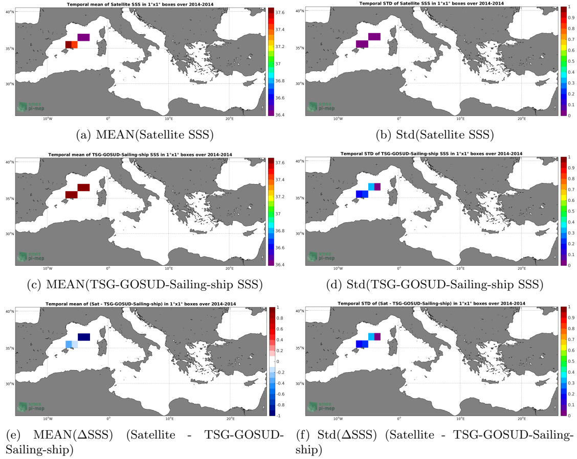
Figure 6: Temporal mean (left) and Std (right) of SSS from Aquarius-L3-OR-V5-MONTHLY-RAIN-MASK-1DEG (top), TSG-GOSUD-Sailing-ship (middle), and of \Delta SSS (Satellite - TSG-GOSUD-Sailing-ship). Only match-up pairs are used to generate these maps.
