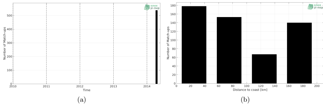
Figure 1: Number of match-ups between TSG-GOSUD-Sailing-ship and Aquarius-L3-OR-V5-MONTHLY-RAIN-MASK-1DEG SSS as a function of time (a) and as function of the distance to coast (b) over the Mediterranean Sea Pi-MEP region and for the full satellite product period.
