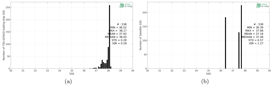
Figure 2: Histograms of SSS from TSG-GOSUD-Sailing-ship (a) and Aquarius-L3-OR-V5-MONTHLY-RAIN-MASK-1DEG (b) considering all match-up pairs per bins of 0.1 over the Mediterranean Sea Pi-MEP region and for the full satellite product period.
