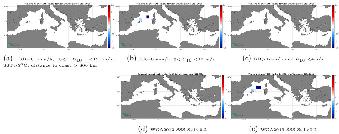
Figure 12: Temporal mean gridded over spatial boxes of size 1^\circ \times 1^\circ of \Delta SSS (Aquarius-L3-OR-V5-MONTHLY-RAIN-MASK-1DEG - TSG-GOSUD-Sailing-ship) for 5 different subdatasets corresponding to:RR=0 mm/h, 3 < U_{10} < 12 m/s, SST >5^\circ\text{C} , distance to coast > 800 km (a), RR=0 mm/h, 3 < U_{10} < 12 m/s (b), RR >1 mm/h and U_{10} < 4 m/s (c), WOA2013 SSS Std <0.2 (d), WOA2013 SSS Std >0.2 (e).
