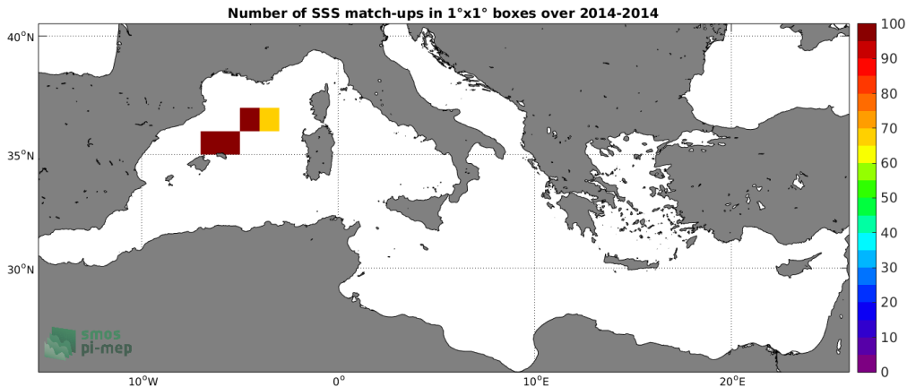
Figure 4: Number of SSS match-ups between TSG-GOSUD-Sailing-ship SSS and the Aquarius-L3-OR-V5-MONTHLY-RAIN-MASK-1DEG SSS product for the Mediterranean Sea Pi-MEP region over 1^\circ \times 1^\circ boxes and for the full satellite product period.
