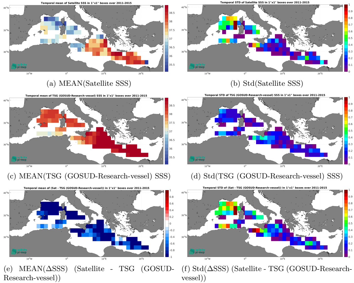
Figure 7: Temporal mean (left) and Std (right) of SSS from Aquarius SSS L3 OR v5 - Monthly - Rain mask (NASA-GSFC) (top), TSG (GOSUD-Research-vessel) (middle), and of \Delta\text{SSS} (Satellite - TSG (GOSUD-Research-vessel)). Only match-up pairs are used to generate these maps.
