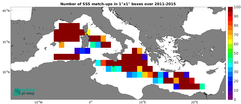
Figure 5: Number of SSS match-ups between TSG (GOSUD-Research-vessel) SSS and the Aquarius SSS L3 OR v5 - Monthly - Rain mask (NASA-GSFC) SSS product for the Mediterranean Sea Pi-MEP region over 1^\circ \times 1^\circ boxes and for the full satellite product period.
