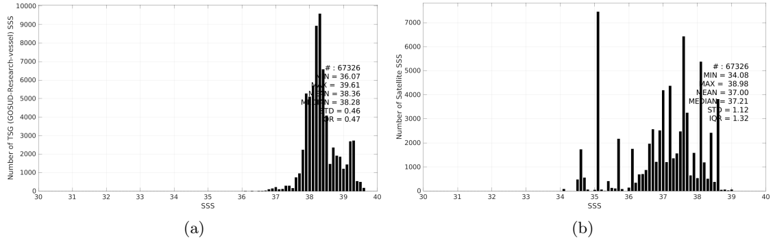
Figure 3: Histograms of SSS from TSG (GOSUD-Research-vessel) (a) and Aquarius SSS L3 OR v5 - Monthly - Rain mask (NASA-GSFC) (b) considering all match-up pairs per bins of 0.1 over the Mediterranean Sea Pi-MEP region and for the full satellite product period.
