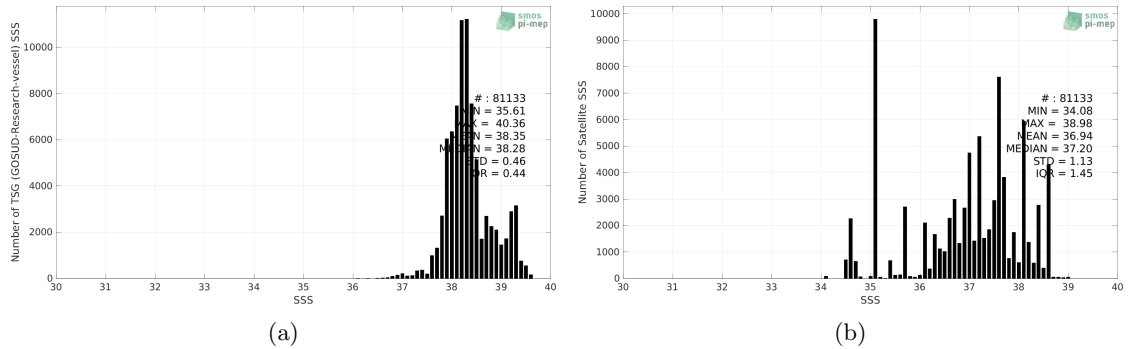
Figure 2: Histograms of SSS from TSG (GOSUD-Research-vessel) (a) and Aquarius SSS L3 OR v5 - Monthly - Rain mask (NASA-GSFC) (b) considering all match-up pairs per bins of 0.1 over the Mediterranean Sea Pi-MEP region and for the full satellite product period.
