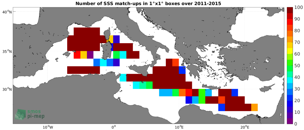
Figure 4: Number of SSS match-ups between TSG (GOSUD-Research-vessel) SSS and the Aquarius SSS L3 OR v5 - Monthly - Rain mask (NASA-GSFC) SSS product for the Mediterranean Sea Pi-MEP region over 1^\circ \times 1^\circ boxes and for the full satellite product period.
