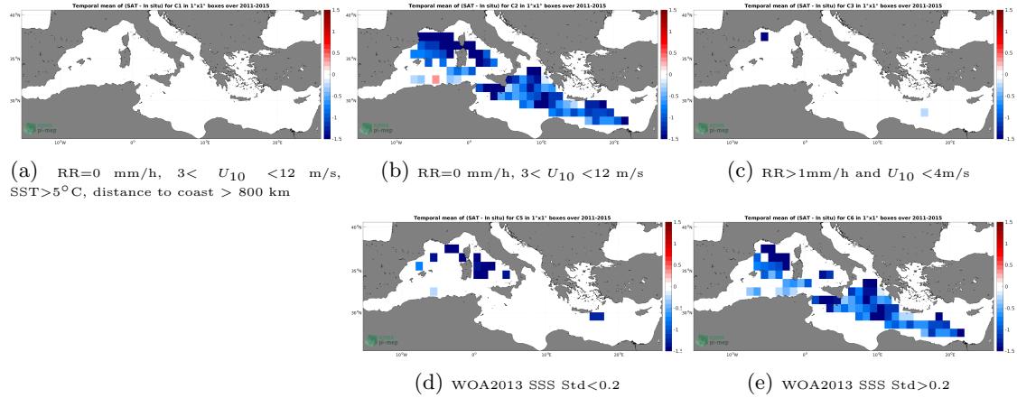
Figure 12: Temporal mean gridded over spatial boxes of size 1^{\circ}\times 1^{\circ} of \Delta SSS (Aquarius SSS L3 OR v5 - Monthly - Rain mask (NASA-GSFC) - TSG (GOSUD-Research-vessel)) for 5 different subdatasets corresponding to:RR=0 mm/h, 3 < U_{10} < 12 m/s, SST >5^{\circ}\text{C} , distance to coast > 800 km (a), RR=0 mm/h, 3 < U_{10} < 12 m/s (b), RR >1 mm/h and U_{10} < 4 m/s (c), WOA2013 SSS Std <0.2 (d), WOA2013 SSS Std >0.2 (e).
