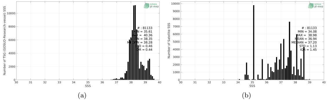
Figure 2: Histograms of SSS from TSG (GOSUD-Research-vessel) (a) and Aquarius SSS L3 OR v5 - Monthly - Rain mask (NASA-GSFC) (b) considering all match-up pairs per bins of 0.1 over the Mediterranean Sea Pi-MEP region and for the full satellite product period.
