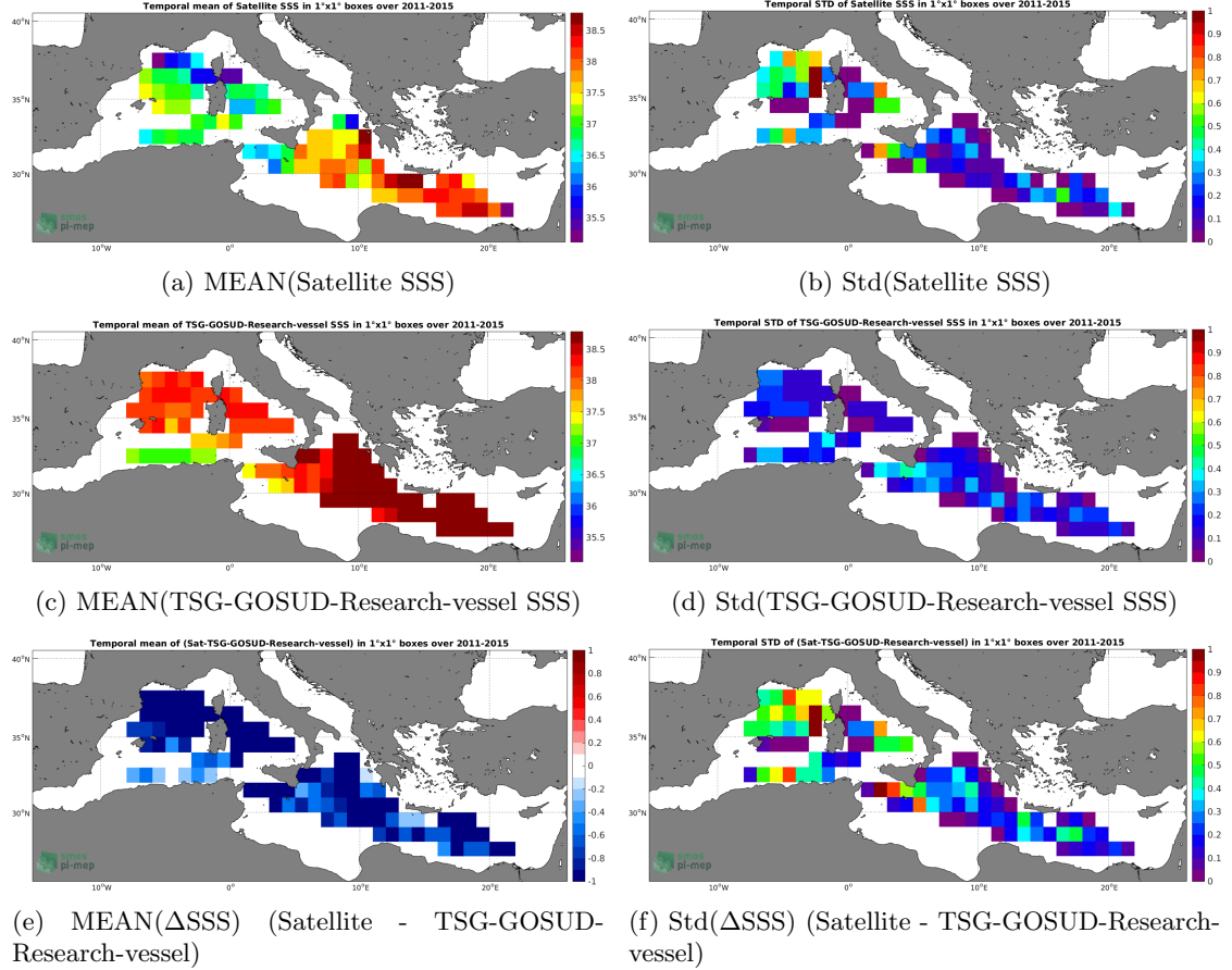
Figure 6: Temporal mean (left) and Std (right) of SSS from Aquarius-L3-OR-V5-MONTHLY-RAIN-MASK-1DEG (top), TSG-GOSUD-Research-vessel (middle), and of \Delta\text{SSS} (Satellite - TSG-GOSUD-Research-vessel). Only match-up pairs are used to generate these maps.
