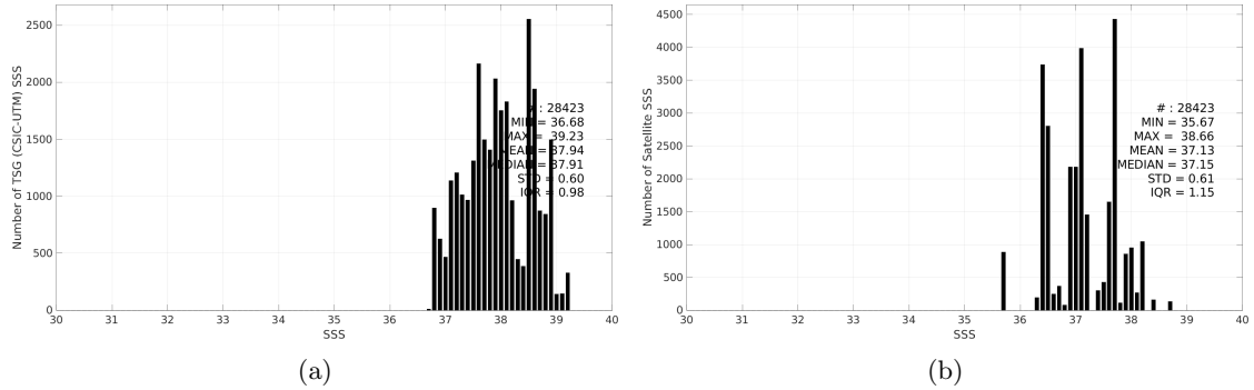
Figure 3: Histograms of SSS from TSG (CSIC-UTM) (a) and Aquarius SSS L3 OR v5 - Monthly - Rain mask (NASA-GSFC) (b) considering all match-up pairs per bins of 0.1 over the Mediterranean Sea Pi-MEP region and for the full satellite product period.
