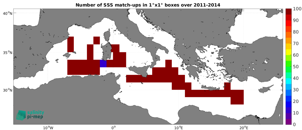
Figure 4: Number of SSS match-ups between TSG (CSIC-UTM) SSS and the Aquarius SSS L3 OR v5 - Monthly - Rain mask (NASA-GSFC) SSS product for the Mediterranean Sea Pi-MEP region over 1^\circ \times 1^\circ boxes and for the full satellite product period.
