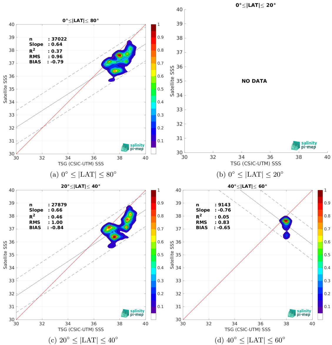
Figure 9: Contour maps of the concentration of Aquarius SSS L3 OR v5 - Monthly - Rain mask (NASA-GSFC) SSS (y-axis) versus TSG (CSIC-UTM) SSS (x-axis) at match-up pairs for different latitude bands. For each plot, the red line shows x=y . The black thin and dashed lines indicate a linear fit through the data cloud and the \pm 95\% confidence levels, respectively. The number match-up pairs n , the slope and R^2 coefficient of the linear fit, the root mean square (RMS) and the mean bias between satellite and in situ data are indicated for each latitude band in each plots.
