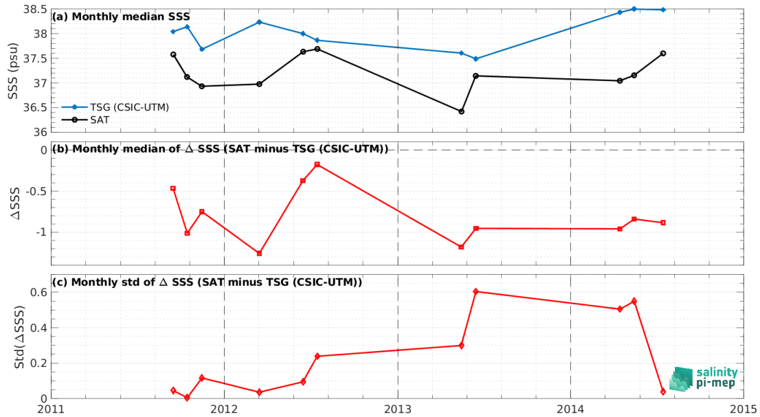
Figure 7: Time series of the monthly median SSS (top), median of \Delta SSS (Satellite - TSG (CSIC-UTM)) and Std of \Delta SSS (Satellite - TSG (CSIC-UTM)) over the Mediterranean Sea Pi-MEP region considering all match-ups collected by the Pi-MEP.
