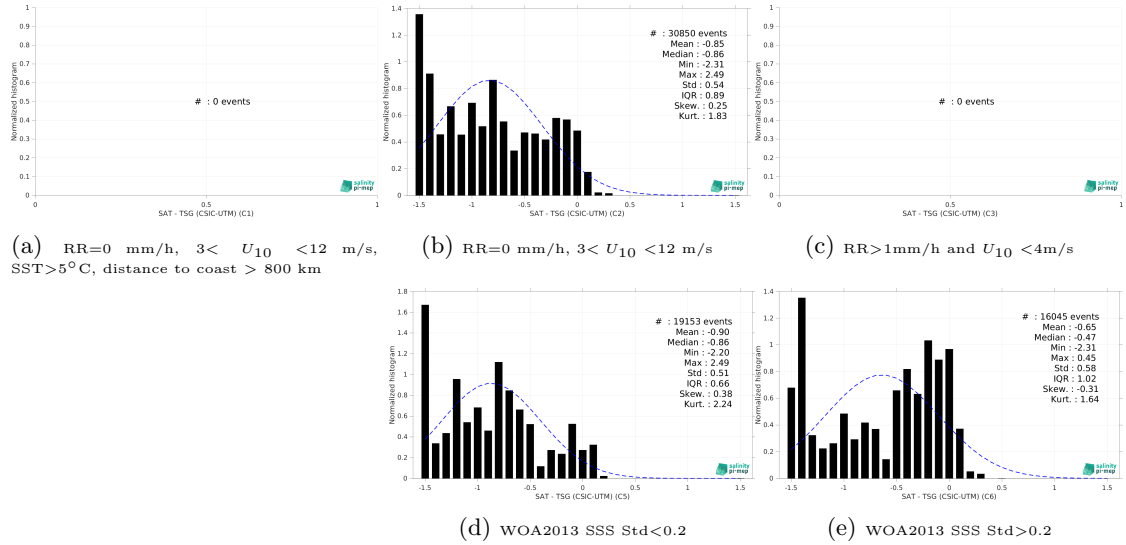
Figure 13: Normalized histogram of \Delta SSS (Aquarius SSS L3 OR v5 - Monthly - Rain mask (NASA-GSFC) - TSG (CSIC-UTM)) for 5 different subdatasets corresponding to: RR=0 mm/h, 3 < U_{10} < 12 m/s, SST > 5°C, distance to coast > 800 km (a), RR=0 mm/h, 3 < U_{10} < 12 m/s (b), RR > 1mm/h and U_{10} < 4 m/s (c), WOA2013 SSS Std < 0.2 (d), WOA2013 SSS Std > 0.2 (e).
