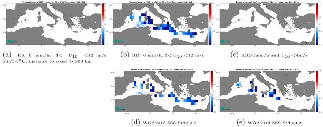
Figure 12: Temporal mean gridded over spatial boxes of size 1^{\circ}\times 1^{\circ} of \Delta\text{SSS} (Aquarius SSS L3 OR v5 - Monthly - Rain mask (NASA-GSFC) - TSG (CSIC-UTM)) for 5 different subdatasets corresponding to:RR=0 mm/h, 3 < U_{10} < 12 m/s, SST >5^{\circ}\text{C} , distance to coast > 800 km (a), RR=0 mm/h, 3 < U_{10} < 12 m/s (b), RR >1 mm/h and U_{10} < 4 m/s (c), WOA2013 SSS Std <0.2 (d), WOA2013 SSS Std >0.2 (e).
