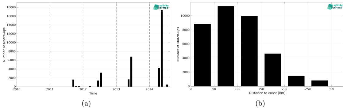
Figure 1: Number of match-ups between TSG (CSIC-UTM) and Aquarius SSS L3 OR v5 - Monthly - Rain mask (NASA-GSFC) SSS as a function of time (a) and as function of the distance to coast (b) over the Mediterranean Sea Pi-MEP region and for the full satellite product period.
