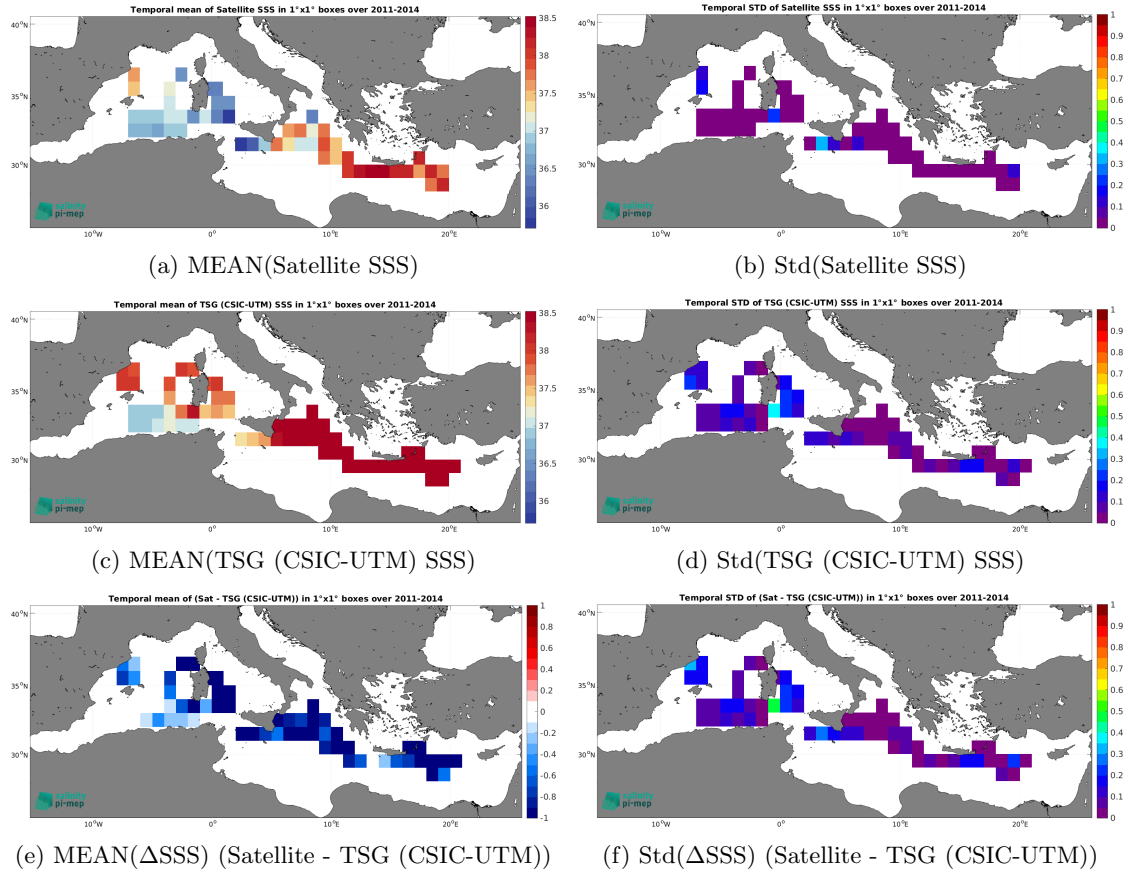
Figure 6: Temporal mean (left) and Std (right) of SSS from Aquarius SSS L3 OR v5 - Monthly - Rain mask (NASA-GSFC) (top), TSG (CSIC-UTM) ( in situ ) dataset (middle), and of \Delta\text{SSS} (Satellite - TSG (CSIC-UTM)). Only match-up pairs are used to generate these maps.
