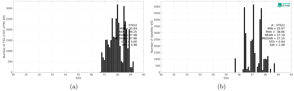
Figure 2: Histograms of SSS from TSG (CSIC-UTM) (a) and Aquarius SSS L3 OR v5 - Monthly - Rain mask (NASA-GSFC) (b) considering all match-up pairs per bins of 0.1 over the Mediterranean Sea Pi-MEP region and for the full satellite product period.
