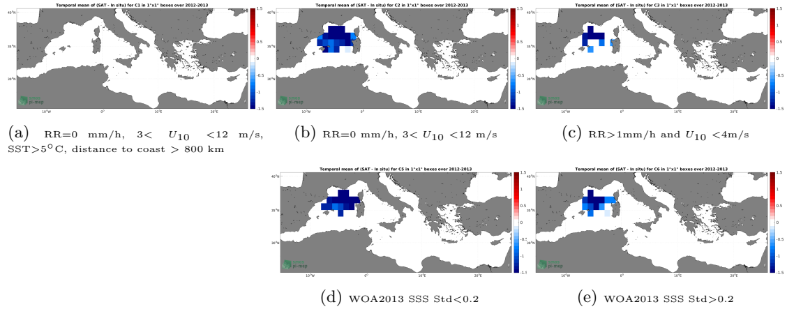
Figure 11: Temporal mean gridded over spatial boxes of size 1^{\circ}\times 1^{\circ} of \Delta\text{SSS} (Aquarius SSS L3 OR v5 - Monthly - Rain mask (NASA-GSFC) - Surface drifters) for 5 different subdatasets corresponding to:RR=0 mm/h, 3 < U_{10} < 12 m/s, SST > 5^{\circ}\text{C} , distance to coast > 800 km (a), RR=0 mm/h, 3 < U_{10} < 12 m/s (b), RR > 1 mm/h and U_{10} < 4 m/s (c), WOA2013 SSS Std < 0.2 (d), WOA2013 SSS Std > 0.2 (e).
