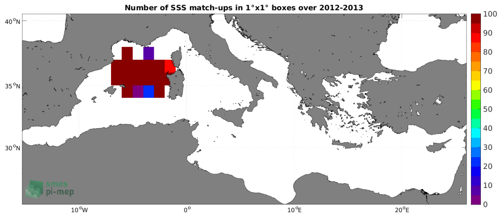
Figure 3: Number of SSS match-ups between Surface drifters SSS and the Aquarius SSS L3 OR v5 - Monthly - Rain mask (NASA-GSFC) SSS product for the Mediterranean Sea Pi-MEP region over 1^\circ \times 1^\circ boxes and for the full satellite product period.
