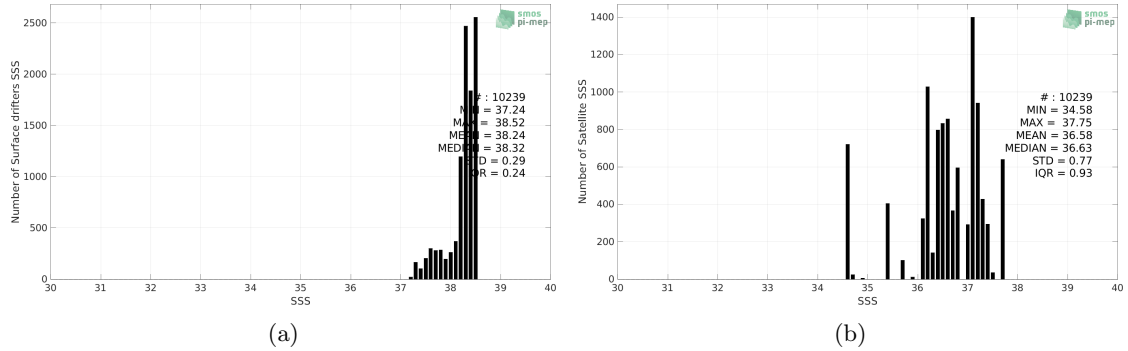
Figure 2: Histograms of SSS from Surface drifters (a) and Aquarius SSS L3 OR v5 - Monthly - Rain mask (NASA-GSFC) (b) considering all match-up pairs per bins of 0.1 over the Mediterranean Sea Pi-MEP region and for the full satellite product period.
