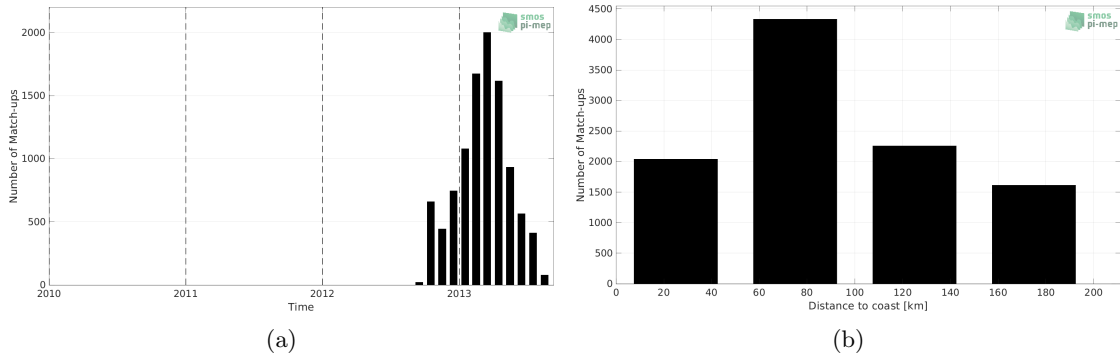
Figure 1: Number of match-ups between Surface drifters and Aquarius SSS L3 OR v5 - Monthly - Rain mask (NASA-GSFC) SSS as a function of time (a) and as function of the distance to coast (b) over the Mediterranean Sea Pi-MEP region and for the full satellite product period.
