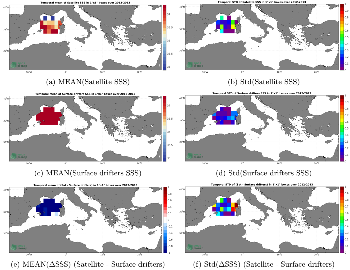
Figure 5: Temporal mean (left) and Std (right) of SSS from Aquarius SSS L3 OR v5 - Monthly - Rain mask (NASA-GSFC) (top), Surface drifters (middle), and of \Delta SSS (Satellite - Surface drifters). Only match-up pairs are used to generate these maps.
