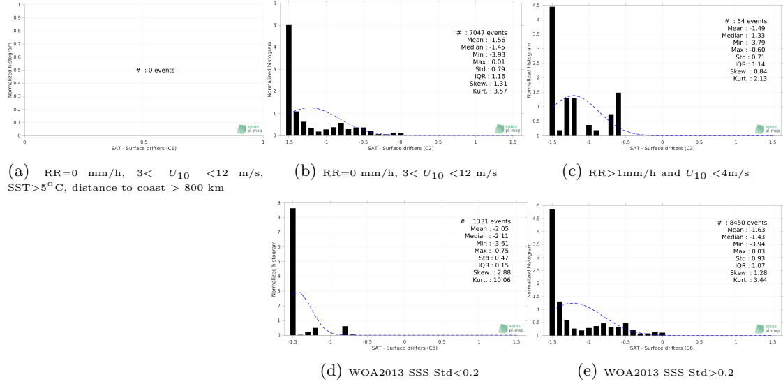
Figure 12: Normalized histogram of \Delta\text{SSS} (Aquarius SSS L3 OR v5 - Monthly - Rain mask (NASA-GSFC) - Surface drifters) for 5 different subdatasets corresponding to: RR=0 mm/h, 3 < U_{10} < 12 m/s, SST > 5^\circ\text{C} , distance to coast > 800 km (a), RR=0 mm/h, 3 < U_{10} < 12 m/s (b), RR > 1\text{mm/h} and U_{10} < 4\text{m/s} (c), WOA2013 SSS Std < 0.2 (d), WOA2013 SSS Std > 0.2 (e).
