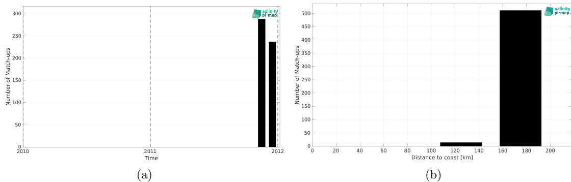
Figure 2: Number of match-ups between TSG (SAMOS) and Aquarius SSS L2 OR v5 (NASA-GSFC) SSS as a function of time (a) and as function of the distance to coast (b) over the Mediterranean Sea Pi-MEP region and for the full satellite product period.
