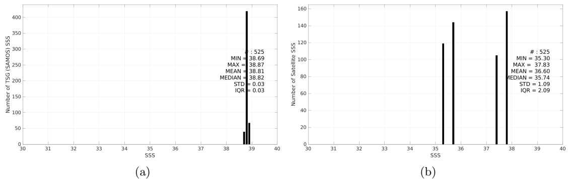
Figure 3: Histograms of SSS from TSG (SAMOS) (a) and Aquarius SSS L2 OR v5 (NASA-GSFC) (b) considering all match-up pairs per bins of 0.1 over the Mediterranean Sea Pi-MEP region and for the full satellite product period.
