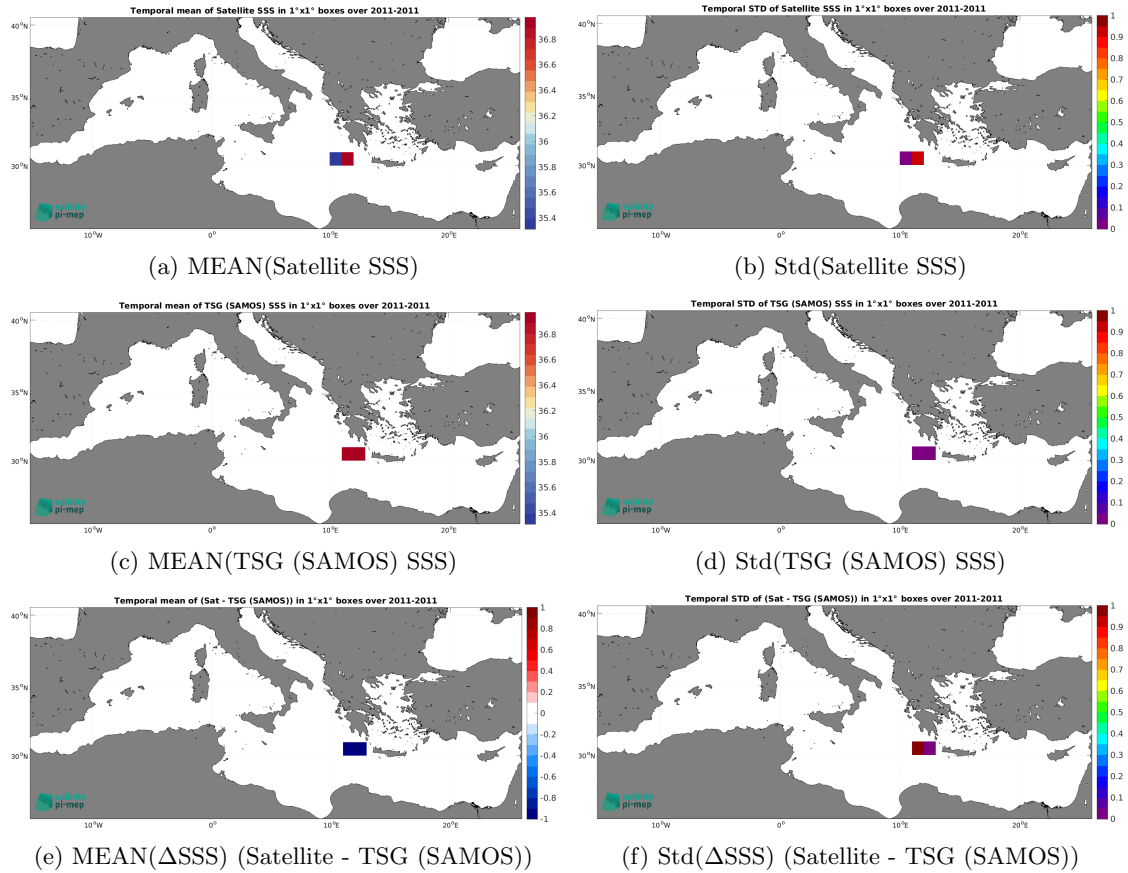
Figure 7: Temporal mean (left) and Std (right) of SSS from Aquarius SSS L2 OR v5 (NASA-GSFC) (top), TSG (SAMOS) ( in situ ) dataset (middle), and of \Delta SSS (Satellite - TSG (SAMOS)). Only match-up pairs are used to generate these maps.
