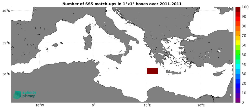
Figure 5: Number of SSS match-ups between TSG (SAMOS) SSS and the Aquarius SSS L2 OR v5 (NASA-GSFC) SSS product for the Mediterranean Sea Pi-MEP region over 1^\circ \times 1^\circ boxes and for the full satellite product period.
