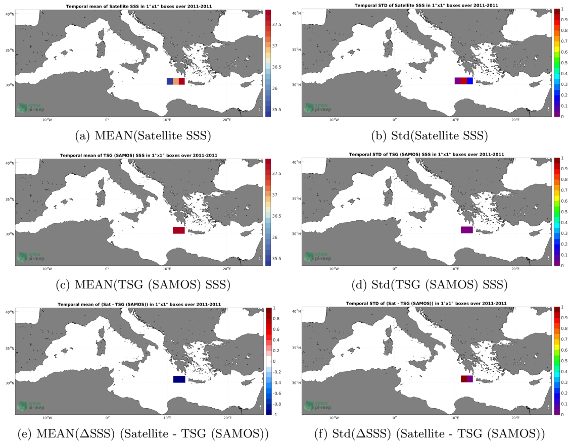
Figure 6: Temporal mean (left) and Std (right) of SSS from Aquarius SSS L2 OR v5 (NASA-GSFC) (top), TSG (SAMOS) ( in situ ) (middle), and of \Delta SSS (Satellite - TSG (SAMOS)). Only match-up pairs are used to generate these maps.
