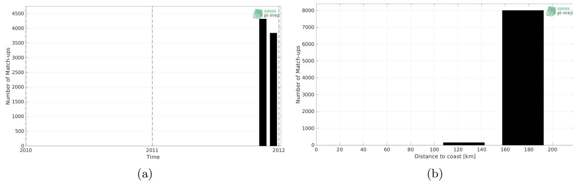
Figure 1: Number of match-ups between TSG (SAMOS) and Aquarius SSS L2 OR v5 (NASA-GSFC) SSS as a function of time (a) and as function of the distance to coast (b) over the Mediterranean Sea Pi-MEP region and for the full satellite product period.
