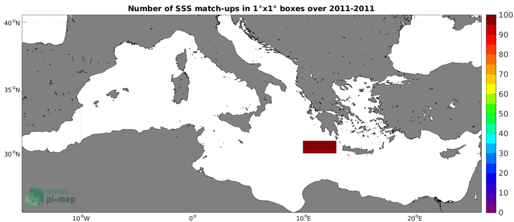
Figure 4: Number of SSS match-ups between TSG (SAMOS) SSS and the Aquarius SSS L2 OR v5 (NASA-GSFC) SSS product for the Mediterranean Sea Pi-MEP region over 1^\circ \times 1^\circ boxes and for the full satellite product period.
