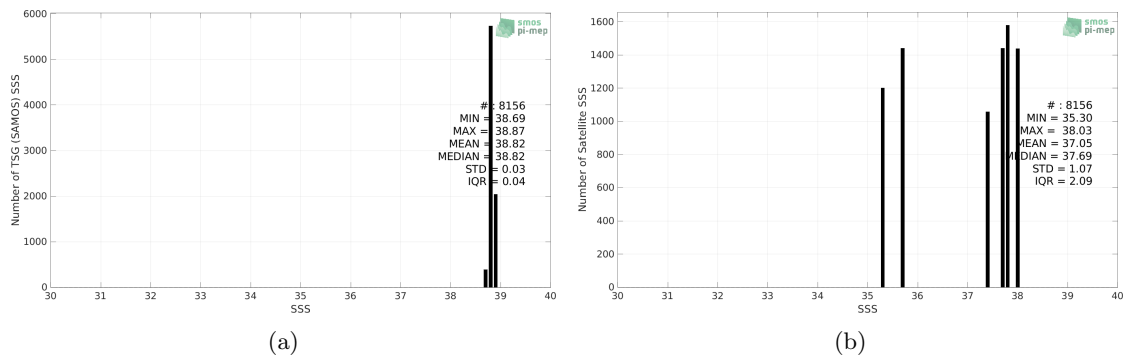
Figure 2: Histograms of SSS from TSG (SAMOS) (a) and Aquarius SSS L2 OR v5 (NASA-GSFC) (b) considering all match-up pairs per bins of 0.1 over the Mediterranean Sea Pi-MEP region and for the full satellite product period.
