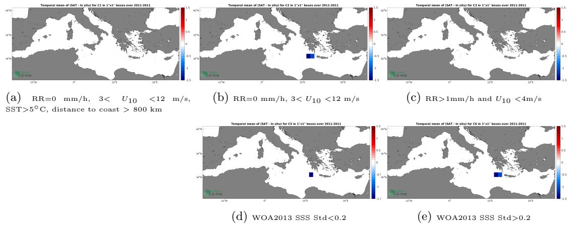
Figure 12: Temporal mean gridded over spatial boxes of size 1^{\circ}\times 1^{\circ} of \Delta\text{SSS} (Aquarius SSS L2 OR v5 (NASA-GSFC) - TSG (SAMOS)) for 5 different subdatasets corresponding to:RR=0 mm/h, 3 < U_{10} < 12 m/s, SST >5^{\circ}\text{C} , distance to coast > 800 km (a), RR=0 mm/h, 3 < U_{10} < 12 m/s (b), RR >1 mm/h and U_{10} < 4 m/s (c), WOA2013 SSS Std <0.2 (d), WOA2013 SSS Std >0.2 (e).
