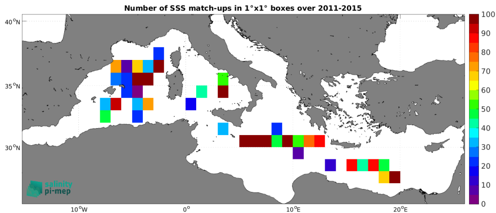
Figure 5: Number of SSS match-ups between TSG (LEGOS-DM) SSS and the Aquarius SSS L2 OR v5 (NASA-GSFC) SSS product for the Mediterranean Sea Pi-MEP region over 1^\circ \times 1^\circ boxes and for the full satellite product period.
