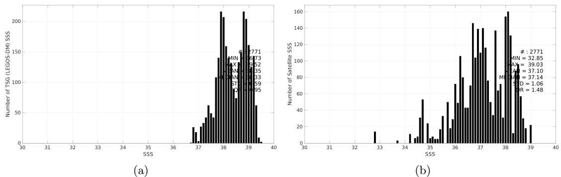
Figure 3: Histograms of SSS from TSG (LEGOS-DM) (a) and Aquarius SSS L2 OR v5 (NASA-GSFC) (b) considering all match-up pairs per bins of 0.1 over the Mediterranean Sea Pi-MEP region and for the full satellite product period.
