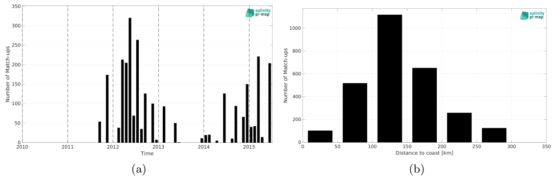
Figure 2: Number of match-ups between TSG (LEGOS-DM) and Aquarius SSS L2 OR v5 (NASA-GSFC) SSS as a function of time (a) and as function of the distance to coast (b) over the Mediterranean Sea Pi-MEP region and for the full satellite product period.
