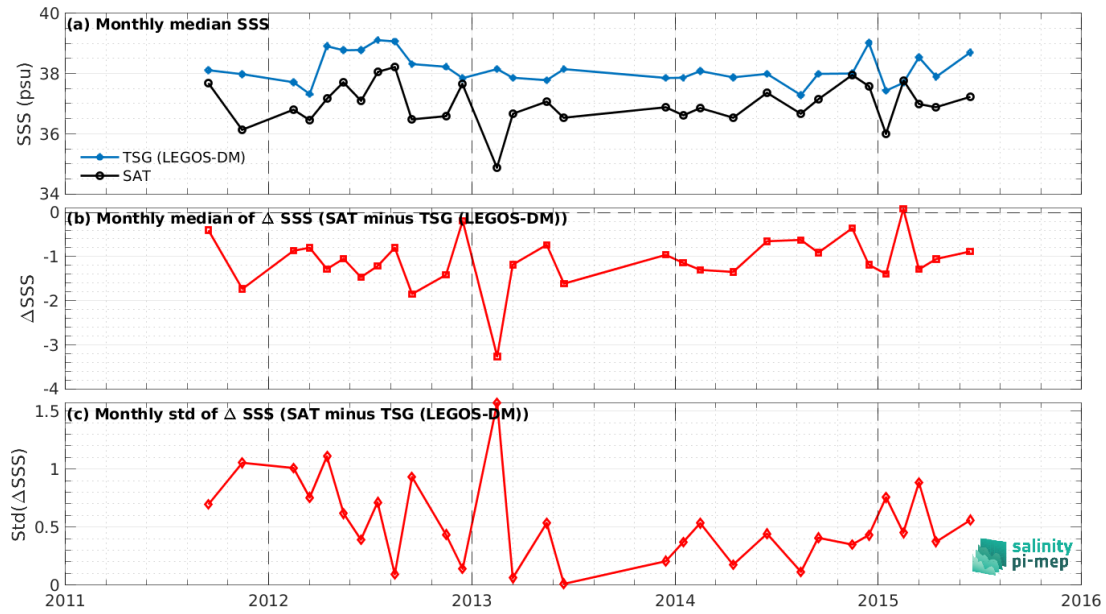
Figure 7: Time series of the monthly median SSS (top), median of \Delta\text{SSS} (Satellite - TSG (LEGOS-DM)) and Std of \Delta\text{SSS} (Satellite - TSG (LEGOS-DM)) over the Mediterranean Sea Pi-MEP region considering all match-ups collected by the Pi-MEP.
