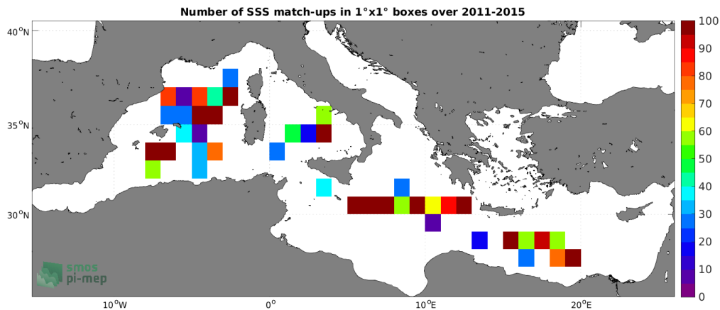
Figure 4: Number of SSS match-ups between TSG (LEGOS-DM) SSS and the Aquarius SSS L2 OR v5 (NASA-GSFC) SSS product for the Mediterranean Sea Pi-MEP region over 1^\circ \times 1^\circ boxes and for the full satellite product period.
