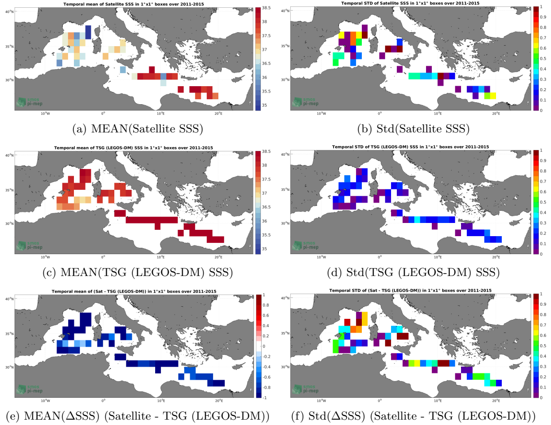
Figure 6: Temporal mean (left) and Std (right) of SSS from Aquarius SSS L2 OR v5 (NASA-GSFC) (top), TSG (LEGOS-DM) (middle), and of \Delta SSS (Satellite - TSG (LEGOS-DM)). Only match-up pairs are used to generate these maps.
