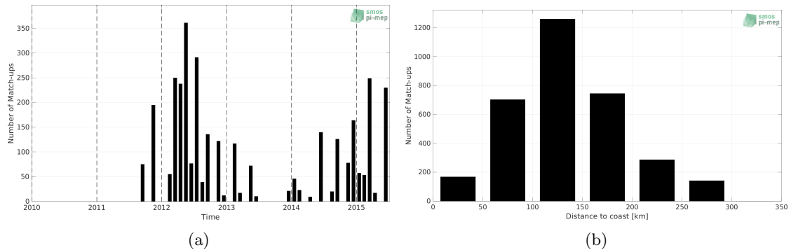
Figure 1: Number of match-ups between TSG (LEGOS-DM) and Aquarius SSS L2 OR v5 (NASA-GSFC) SSS as a function of time (a) and as function of the distance to coast (b) over the Mediterranean Sea Pi-MEP region and for the full satellite product period.
