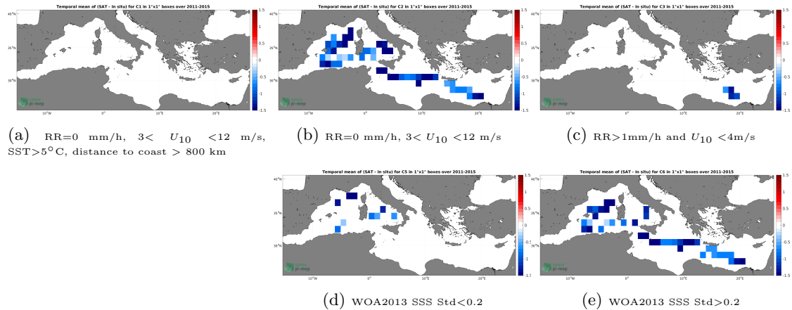
Figure 12: Temporal mean gridded over spatial boxes of size 1^\circ \times 1^\circ of \Delta SSS (Aquarius SSS L2 OR v5 (NASA-GSFC) - TSG (LEGOS-DM)) for 5 different subdatasets corresponding to:RR=0 mm/h, 3 < U_{10} < 12 m/s, SST >5^\circ\text{C} , distance to coast > 800 km (a), RR=0 mm/h, 3 < U_{10} < 12 m/s (b), RR >1 mm/h and U_{10} < 4 m/s (c), WOA2013 SSS Std <0.2 (d), WOA2013 SSS Std >0.2 (e).
