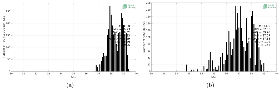
Figure 2: Histograms of SSS from TSG (LEGOS-DM) (a) and Aquarius SSS L2 OR v5 (NASA-GSFC) (b) considering all match-up pairs per bins of 0.1 over the Mediterranean Sea Pi-MEP region and for the full satellite product period.
