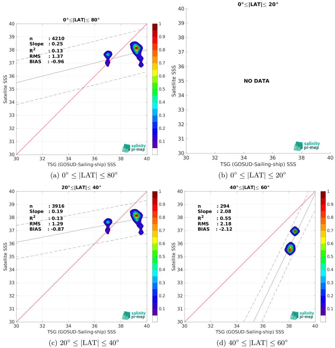
Figure 10: Contour maps of the concentration of Aquarius SSS L2 OR v5 (NASA-GSFC) SSS (y-axis) versus TSG (GOSUD-Sailing-ship) SSS (x-axis) at match-up pairs for different latitude bands. For each plot, the red line shows x=y . The black thin and dashed lines indicate a linear fit through the data cloud and the \pm 95\% confidence levels, respectively. The number match-up pairs n , the slope and R^2 coefficient of the linear fit, the root mean square (RMS) and the mean bias between satellite and in situ data are indicated for each latitude band in each plots.
