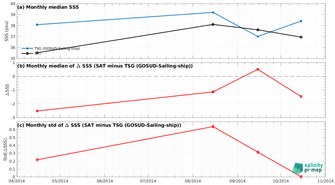
Figure 8: Time series of the monthly median SSS (top), median of \Delta SSS (Satellite - TSG (GOSUD-Sailing-ship)) and Std of \Delta SSS (Satellite - TSG (GOSUD-Sailing-ship)) over the Mediterranean Sea Pi-MEP region considering all match-ups collected by the Pi-MEP.
