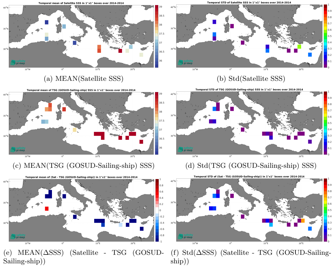
Figure 7: Temporal mean (left) and Std (right) of SSS from Aquarius SSS L2 OR v5 (NASA-GSFC) (top), TSG (GOSUD-Sailing-ship) (middle), and of \Delta SSS (Satellite - TSG (GOSUD-Sailing-ship)). Only match-up pairs are used to generate these maps.
