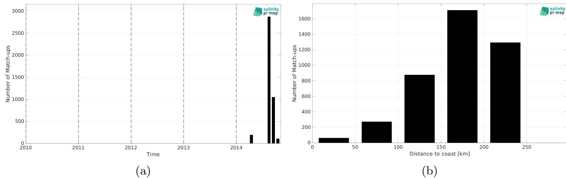
Figure 2: Number of match-ups between TSG (GOSUD-Sailing-ship) and Aquarius SSS L2 OR v5 (NASA-GSFC) SSS as a function of time (a) and as function of the distance to coast (b) over the Mediterranean Sea Pi-MEP region and for the full satellite product period.
