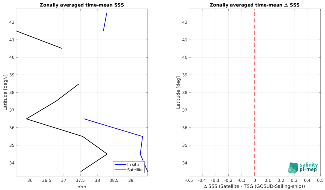
Figure 9: Left panel: Zonal mean SSS from Aquarius SSS L2 OR v5 (NASA-GSFC) satellite product (black) and from TSG (GOSUD-Sailing-ship) (blue). Right panel: Zonal mean of \Delta SSS (Satellite - TSG (GOSUD-Sailing-ship)) for all the collected Pi-MEP match-up pairs estimated over the full satellite product period.
