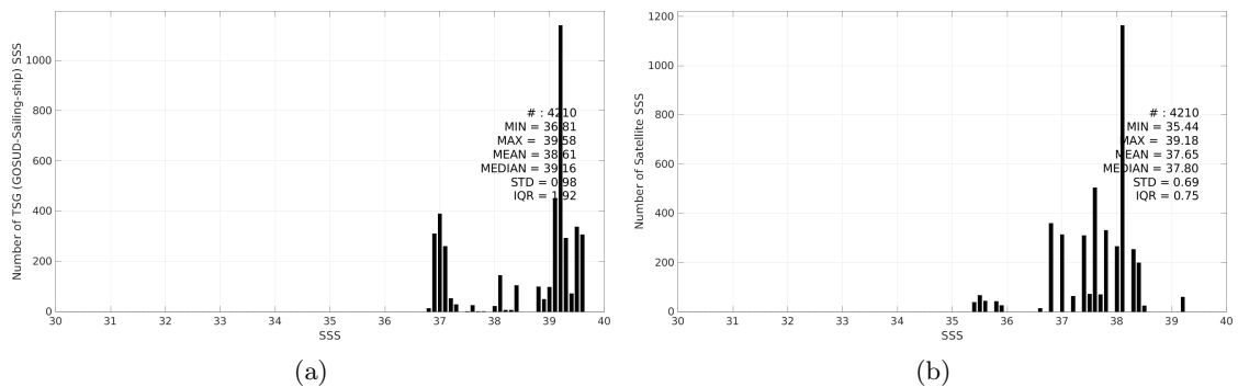
Figure 3: Histograms of SSS from TSG (GOSUD-Sailing-ship) (a) and Aquarius SSS L2 OR v5 (NASA-GSFC) (b) considering all match-up pairs per bins of 0.1 over the Mediterranean Sea Pi-MEP region and for the full satellite product period.
