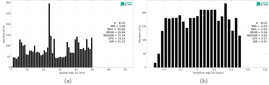
Figure 6: Histograms of the spatial (a) and temporal (b) lags between the location/time of the TSG (GOSUD-Sailing-ship) measurement and the date of the corresponding Aquarius SSS L2 OR v5 (NASA-GSFC) SSS pixel.
