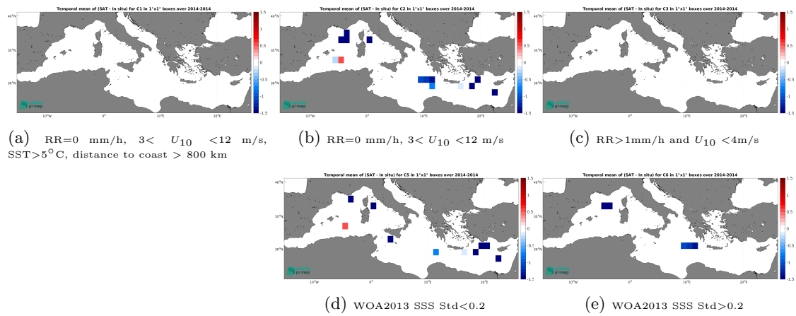
Figure 14: Temporal mean gridded over spatial boxes of size 1^\circ \times 1^\circ of \Delta SSS (Aquarius SSS L2 OR v5 (NASA-GSFC) - TSG (GOSUD-Sailing-ship)) for 5 different subdatasets corresponding to:RR=0 mm/h, 3 < U_{10} < 12 m/s, SST>5°C, distance to coast > 800 km (a), RR=0 mm/h, 3 < U_{10} < 12 m/s (b), RR>1mm/h and U_{10} < 4 m/s (c), WOA2013 SSS Std<0.2 (d), WOA2013 SSS Std>0.2 (e).
