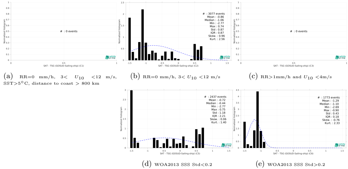
Figure 15: Normalized histogram of \Delta SSS (Aquarius SSS L2 OR v5 (NASA-GSFC) - TSG (GOSUD-Sailing-ship)) for 5 different subdatasets corresponding to: RR=0 mm/h, 3 < U_{10} < 12 m/s, SST>5°C, distance to coast > 800 km (a), RR=0 mm/h, 3 < U_{10} < 12 m/s (b), RR>1mm/h and U_{10} < 4 m/s (c), WOA2013 SSS Std<0.2 (d), WOA2013 SSS Std>0.2 (e).
