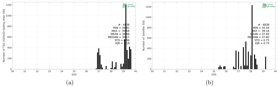
Figure 2: Histograms of SSS from TSG (GOSUD-Sailing-ship) (a) and Aquarius SSS L2 OR v5 (NASA-GSFC) (b) considering all match-up pairs per bins of 0.1 over the Mediterranean Sea Pi-MEP region and for the full satellite product period.
