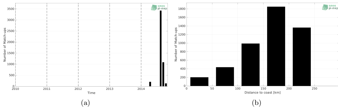
Figure 1: Number of match-ups between TSG (GOSUD-Sailing-ship) and Aquarius SSS L2 OR v5 (NASA-GSFC) SSS as a function of time (a) and as function of the distance to coast (b) over the Mediterranean Sea Pi-MEP region and for the full satellite product period.
