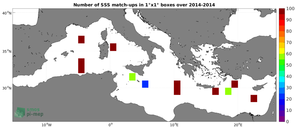
Figure 4: Number of SSS match-ups between TSG (GOSUD-Sailing-ship) SSS and the Aquarius SSS L2 OR v5 (NASA-GSFC) SSS product for the Mediterranean Sea Pi-MEP region over 1^\circ \times 1^\circ boxes and for the full satellite product period.
