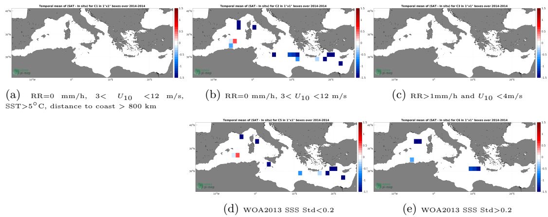
Figure 12: Temporal mean gridded over spatial boxes of size 1^\circ \times 1^\circ of \Delta SSS (Aquarius SSS L2 OR v5 (NASA-GSFC) - TSG (GOSUD-Sailing-ship)) for 5 different subdatasets corresponding to:RR=0 mm/h, 3 < U_{10} < 12 m/s, SST>5°C, distance to coast > 800 km (a), RR=0 mm/h, 3 < U_{10} < 12 m/s (b), RR>1mm/h and U_{10} < 4 m/s (c), WOA2013 SSS Std<0.2 (d), WOA2013 SSS Std>0.2 (e).
