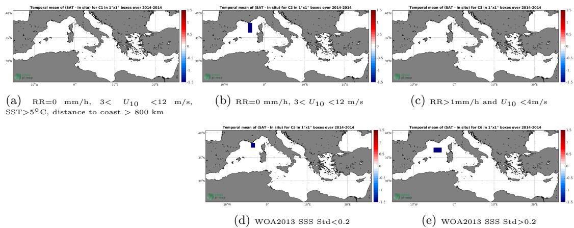
Figure 12: Temporal mean gridded over spatial boxes of size 1^\circ \times 1^\circ of \Delta SSS (Aquarius-L2-OR-V5 - TSG-GOSUD-Sailing-ship) for 5 different subdatasets corresponding to:RR=0 mm/h, 3 < U_{10} < 12 m/s, SST >5^\circ\text{C} , distance to coast > 800 km (a), RR=0 mm/h, 3 < U_{10} < 12 m/s (b), RR >1 mm/h and U_{10} < 4 m/s (c), WOA2013 SSS Std <0.2 (d), WOA2013 SSS Std >0.2 (e).
