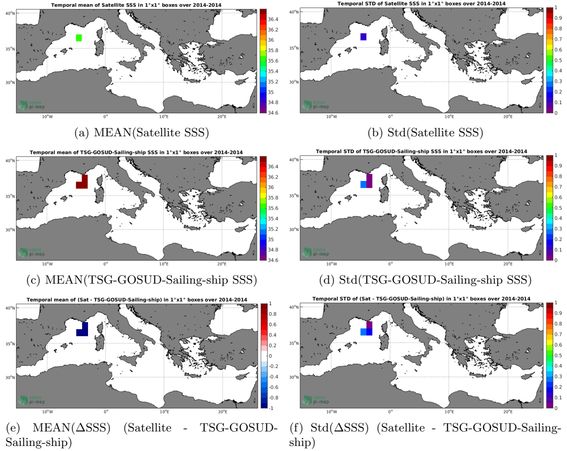
Figure 6: Temporal mean (left) and Std (right) of SSS from Aquarius-L2-OR-V5 (top), TSG-GOSUD-Sailing-ship (middle), and of \Delta SSS (Satellite - TSG-GOSUD-Sailing-ship). Only match-up pairs are used to generate these maps.
