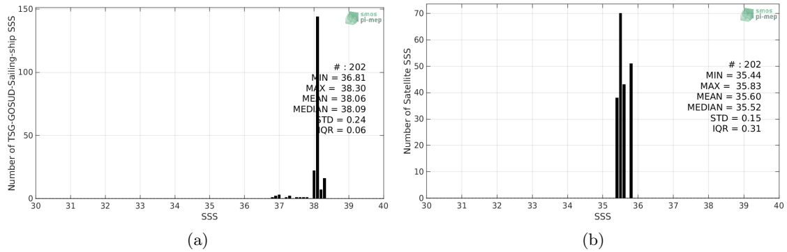
Figure 2: Histograms of SSS from TSG-GOSUD-Sailing-ship (a) and Aquarius-L2-OR-V5 (b) considering all match-up pairs per bins of 0.1 over the Mediterranean Sea Pi-MEP region and for the full satellite product period.
