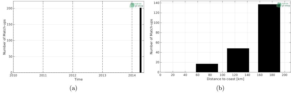
Figure 1: Number of match-ups between TSG-GOSUD-Sailing-ship and Aquarius-L2-OR-V5 SSS as a function of time (a) and as function of the distance to coast (b) over the Mediterranean Sea Pi-MEP region and for the full satellite product period.
