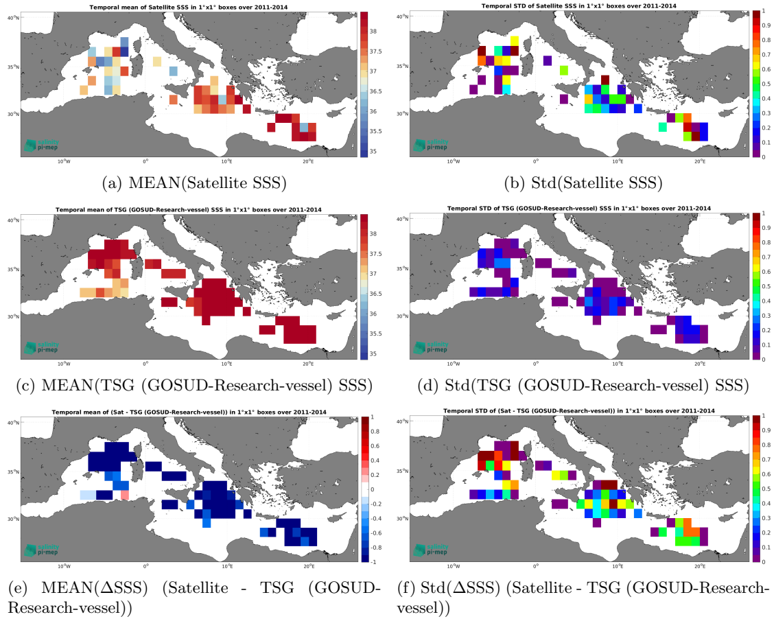
Figure 7: Temporal mean (left) and Std (right) of SSS from Aquarius SSS L2 OR v5 (NASA-GSFC) (top), TSG (GOSUD-Research-vessel) (middle), and of \Delta SSS (Satellite - TSG (GOSUD-Research-vessel)). Only match-up pairs are used to generate these maps.
