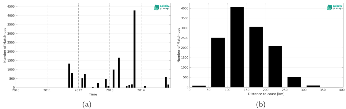
Figure 2: Number of match-ups between TSG (GOSUD-Research-vessel) and Aquarius SSS L2 OR v5 (NASA-GSFC) SSS as a function of time (a) and as function of the distance to coast (b) over the Mediterranean Sea Pi-MEP region and for the full satellite product period.
