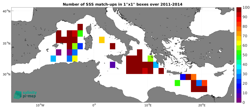
Figure 5: Number of SSS match-ups between TSG (GOSUD-Research-vessel) SSS and the Aquarius SSS L2 OR v5 (NASA-GSFC) SSS product for the Mediterranean Sea Pi-MEP region over 1^\circ \times 1^\circ boxes and for the full satellite product period.
