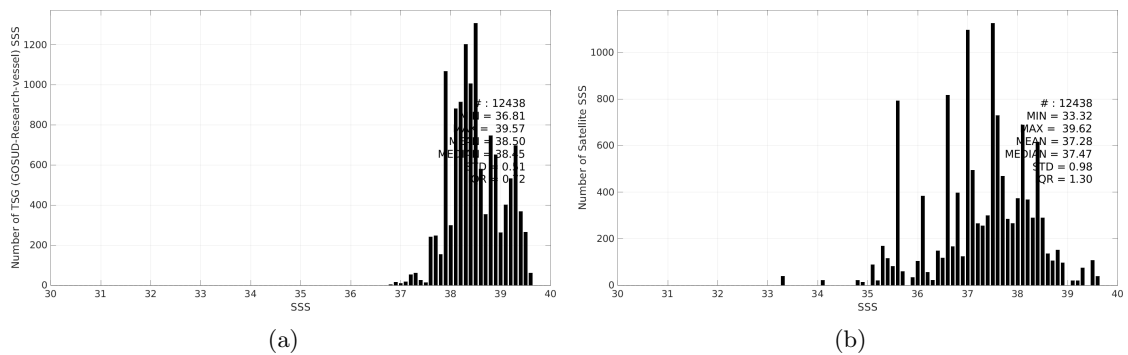
Figure 3: Histograms of SSS from TSG (GOSUD-Research-vessel) (a) and Aquarius SSS L2 OR v5 (NASA-GSFC) (b) considering all match-up pairs per bins of 0.1 over the Mediterranean Sea Pi-MEP region and for the full satellite product period.
