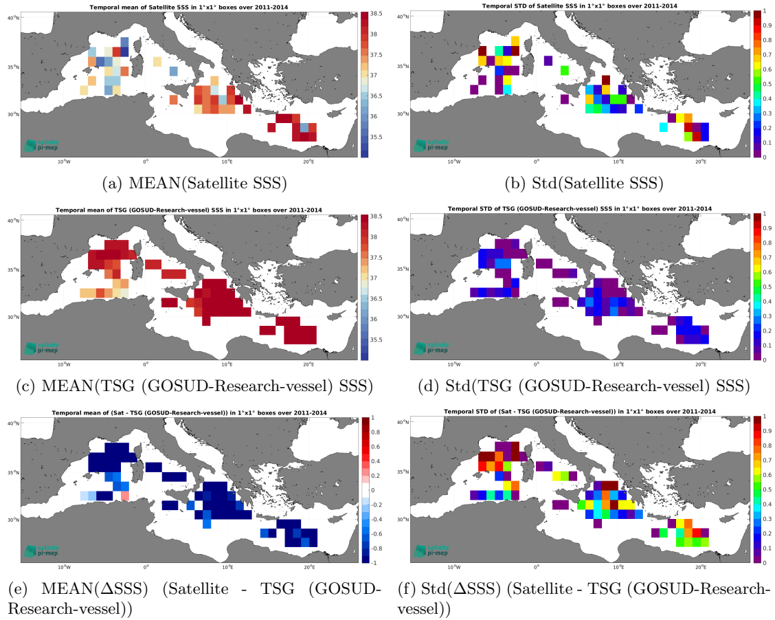
Figure 6: Temporal mean (left) and Std (right) of SSS from Aquarius SSS L2 OR v5 (NASA-GSFC) (top), TSG (GOSUD-Research-vessel) (middle), and of \Delta SSS (Satellite - TSG (GOSUD-Research-vessel)). Only match-up pairs are used to generate these maps.
