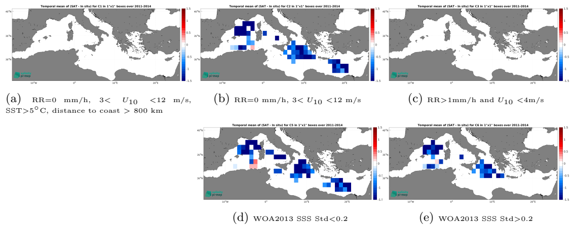
Figure 12: Temporal mean gridded over spatial boxes of size 1^\circ \times 1^\circ of \Delta SSS (Aquarius SSS L2 OR v5 (NASA-GSFC) - TSG (GOSUD-Research-vessel)) for 5 different subdatasets corresponding to:RR=0 mm/h, 3 < U_{10} < 12 m/s, SST>5°C, distance to coast > 800 km (a), RR=0 mm/h, 3 < U_{10} < 12 m/s (b), RR>1mm/h and U_{10} < 4 m/s (c), WOA2013 SSS Std<0.2 (d), WOA2013 SSS Std>0.2 (e).
