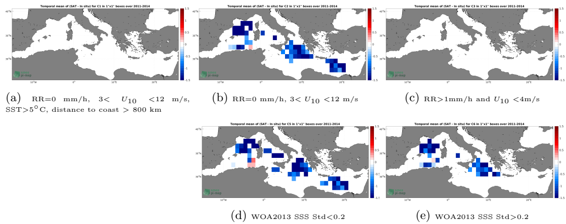
Figure 12: Temporal mean gridded over spatial boxes of size 1^\circ \times 1^\circ of \Delta\text{SSS} (Aquarius SSS L2 OR v5 (NASA-GSFC) - TSG (GOSUD-Research-vessel)) for 5 different subdatasets corresponding to:RR=0 mm/h, 3 < U_{10} < 12 m/s, SST>5°C, distance to coast > 800 km (a), RR=0 mm/h, 3 < U_{10} < 12 m/s (b), RR>1mm/h and U_{10} < 4 m/s (c), WOA2013 SSS Std<0.2 (d), WOA2013 SSS Std>0.2 (e).
