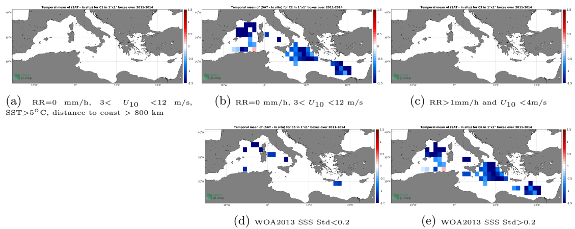
Figure 12: Temporal mean gridded over spatial boxes of size 1^\circ \times 1^\circ of \Delta SSS (Aquarius SSS L2 OR v5 (NASA-GSFC) - TSG (GOSUD-Research-vessel)) for 5 different subdatasets corresponding to:RR=0 mm/h, 3 < U_{10} < 12 m/s, SST > 5°C, distance to coast > 800 km (a), RR=0 mm/h, 3 < U_{10} < 12 m/s (b), RR > 1mm/h and U_{10} < 4 m/s (c), WOA2013 SSS Std < 0.2 (d), WOA2013 SSS Std > 0.2 (e).
