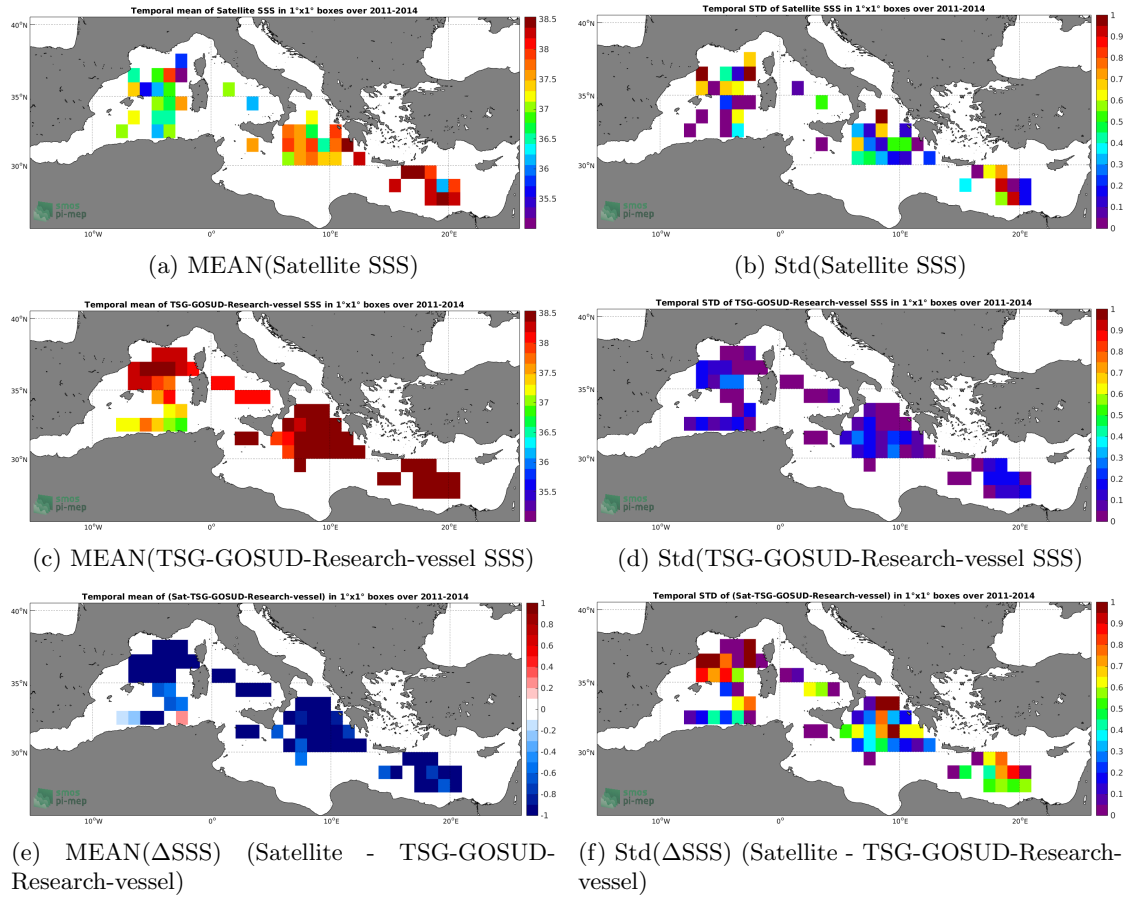
Figure 6: Temporal mean (left) and Std (right) of SSS from Aquarius-L2-OR-V5 (top), TSG-GOSUD-Research-vessel (middle), and of \Delta SSS (Satellite - TSG-GOSUD-Research-vessel). Only match-up pairs are used to generate these maps.
