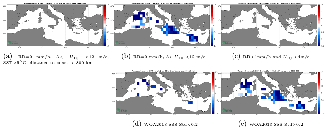
Figure 12: Temporal mean gridded over spatial boxes of size 1^\circ \times 1^\circ of \Delta SSS (Aquarius-L2-OR-V5 - TSG-GOSUD-Research-vessel) for 5 different subdatasets corresponding to:RR=0 mm/h, 3 < U_{10} < 12 m/s, SST >5^\circ\text{C} , distance to coast > 800 km (a), RR=0 mm/h, 3 < U_{10} < 12 m/s (b), RR >1 mm/h and U_{10} < 4 m/s (c), WOA2013 SSS Std <0.2 (d), WOA2013 SSS Std >0.2 (e).
