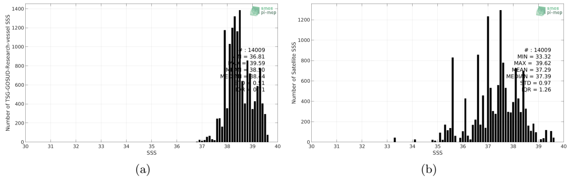
Figure 2: Histograms of SSS from TSG-GOSUD-Research-vessel (a) and Aquarius-L2-OR-V5 (b) considering all match-up pairs per bins of 0.1 over the Mediterranean Sea Pi-MEP region and for the full satellite product period.
