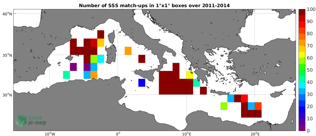
Figure 4: Number of SSS match-ups between TSG-GOSUD-Research-vessel SSS and the Aquarius-L2-OR-V5 SSS product for the Mediterranean Sea Pi-MEP region over 1^\circ \times 1^\circ boxes and for the full satellite product period.
