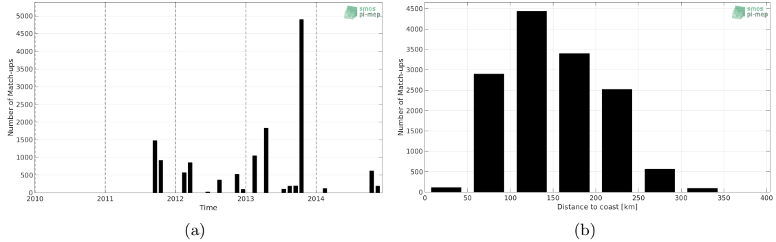
Figure 1: Number of match-ups between TSG-GOSUD-Research-vessel and Aquarius-L2-OR-V5 SSS as a function of time (a) and as function of the distance to coast (b) over the Mediterranean Sea Pi-MEP region and for the full satellite product period.
