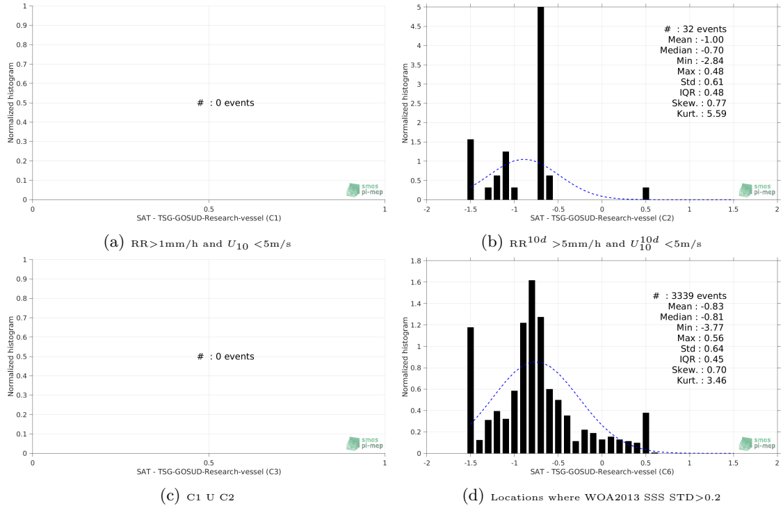
Figure 13: Normalized histogram of \Delta\text{SSS} (Aquarius-L2-OR-V5 - TSG-GOSUD-Research-vessel) for 6 different subdatasets corresponding to: RR > 1\text{mm/h} and U_{10} < 5\text{m/s} (a), RR^{10d} > 5\text{mm/h} and U_{10}^{10d} < 5\text{m/s} (b), C1 \cup C2 (c), Locations where WOA2013 SSS STD > 0.2 (d).
