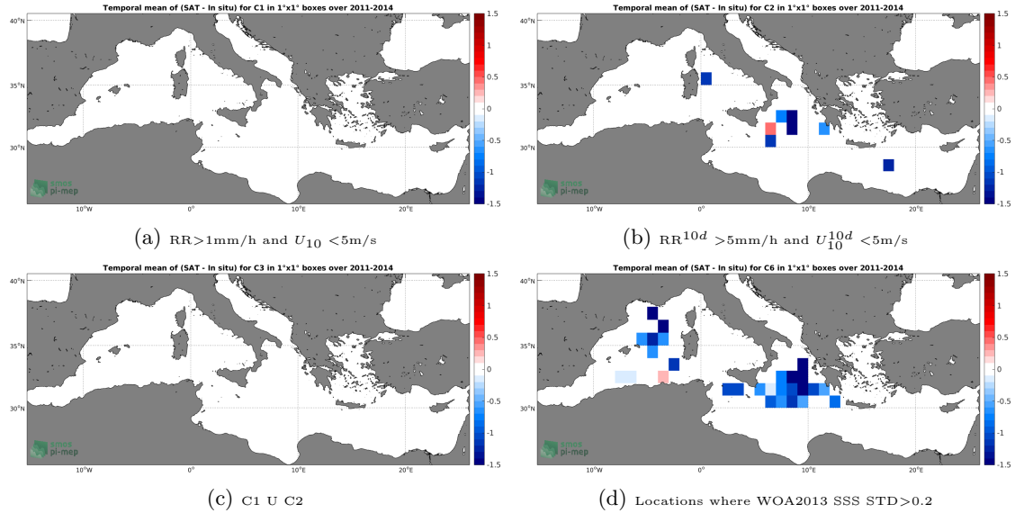
Figure 12: Temporal mean gridded over spatial boxes of size 1^\circ \times 1^\circ of \Delta SSS (Aquarius-L2-OR-V5 - TSG-GOSUD-Research-vessel) for 4 different subdatasets corresponding to: RR > 1mm/h and U_{10} < 5\text{m/s} (a), RR^{10d} > 5\text{mm/h} and U_{10d} < 5\text{m/s} (b), C1 U C2 (c), Locations where WOA2013 SSS STD > 0.2 (d).
