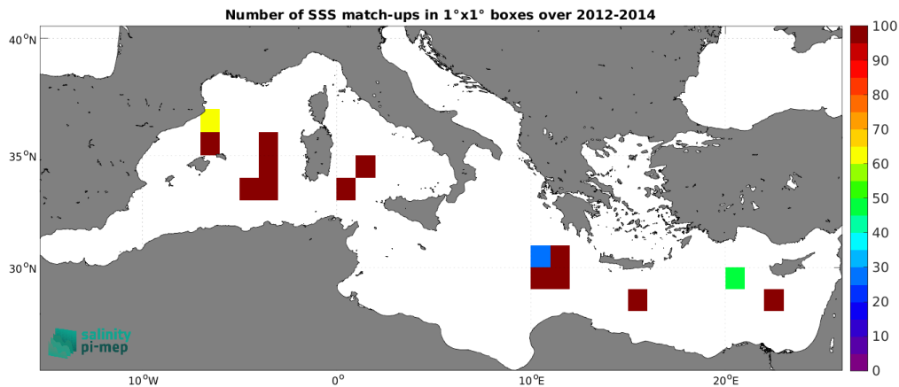
Figure 5: Number of SSS match-ups between TSG (CSIC-UTM) SSS and the Aquarius SSS L2 OR v5 (NASA-GSFC) SSS product for the Mediterranean Sea Pi-MEP region over 1^\circ \times 1^\circ boxes and for the full satellite product period.
