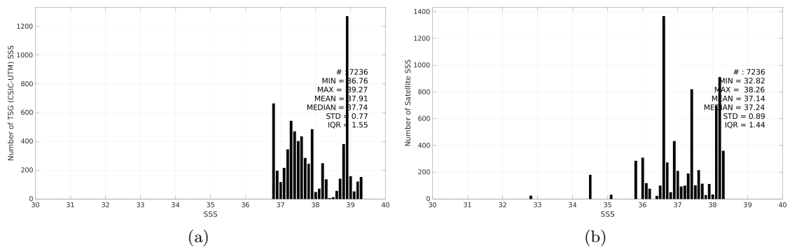
Figure 3: Histograms of SSS from TSG (CSIC-UTM) (a) and Aquarius SSS L2 OR v5 (NASA-GSFC) (b) considering all match-up pairs per bins of 0.1 over the Mediterranean Sea Pi-MEP region and for the full satellite product period.
