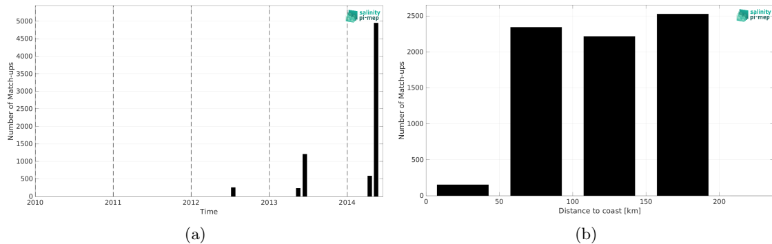
Figure 2: Number of match-ups between TSG (CSIC-UTM) and Aquarius SSS L2 OR v5 (NASA-GSFC) SSS as a function of time (a) and as function of the distance to coast (b) over the Mediterranean Sea Pi-MEP region and for the full satellite product period.
