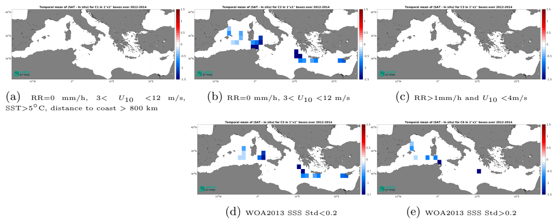
Figure 14: Temporal mean gridded over spatial boxes of size 1^\circ \times 1^\circ of \Delta SSS (Aquarius SSS L2 OR v5 (NASA-GSFC) - TSG (CSIC-UTM)) for 5 different subdatasets corresponding to:RR=0 mm/h, 3 < U_{10} < 12 m/s, SST >5^\circ\text{C} , distance to coast > 800 km (a), RR=0 mm/h, 3 < U_{10} < 12 m/s (b), RR >1 mm/h and U_{10} < 4 m/s (c), WOA2013 SSS Std <0.2 (d), WOA2013 SSS Std >0.2 (e).
