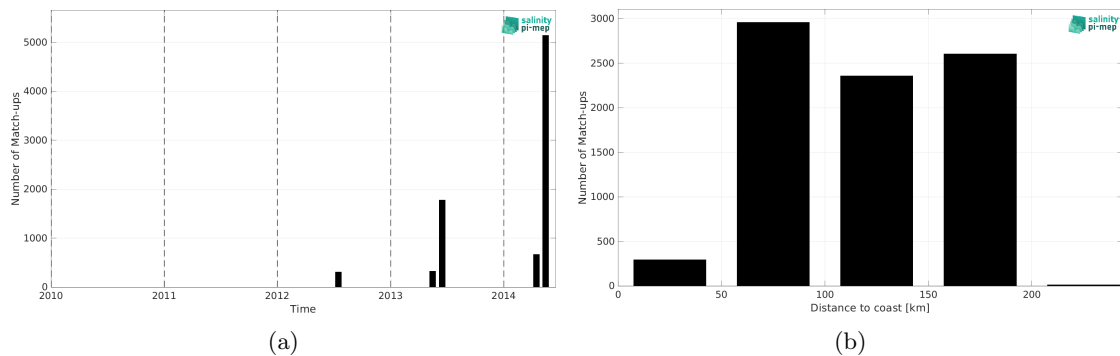
Figure 1: Number of match-ups between TSG (CSIC-UTM) and Aquarius SSS L2 OR v5 (NASA-GSFC) SSS as a function of time (a) and as function of the distance to coast (b) over the Mediterranean Sea Pi-MEP region and for the full satellite product period.
