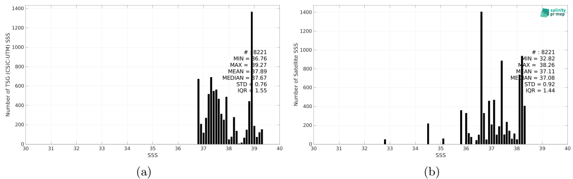
Figure 2: Histograms of SSS from TSG (CSIC-UTM) (a) and Aquarius SSS L2 OR v5 (NASA-GSFC) (b) considering all match-up pairs per bins of 0.1 over the Mediterranean Sea Pi-MEP region and for the full satellite product period.
