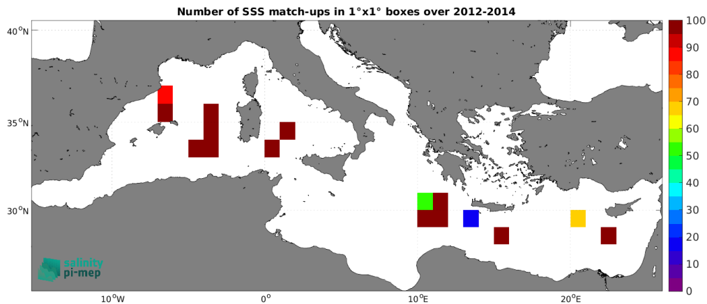
Figure 4: Number of SSS match-ups between TSG (CSIC-UTM) SSS and the Aquarius SSS L2 OR v5 (NASA-GSFC) SSS product for the Mediterranean Sea Pi-MEP region over 1^\circ \times 1^\circ boxes and for the full satellite product period.
