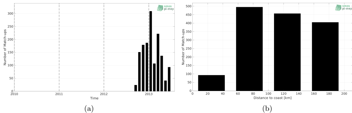
Figure 1: Number of match-ups between Surface drifters and Aquarius SSS L2 OR v5 (NASA-GSFC) SSS as a function of time (a) and as function of the distance to coast (b) over the Mediterranean Sea Pi-MEP region and for the full satellite product period.
