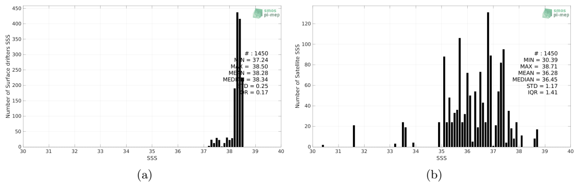
Figure 2: Histograms of SSS from Surface drifters (a) and Aquarius SSS L2 OR v5 (NASA-GSFC) (b) considering all match-up pairs per bins of 0.1 over the Mediterranean Sea Pi-MEP region and for the full satellite product period.
