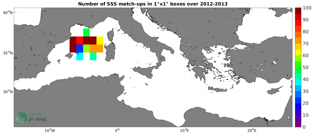
Figure 3: Number of SSS match-ups between Surface drifters SSS and the Aquarius SSS L2 OR v5 (NASA-GSFC) SSS product for the Mediterranean Sea Pi-MEP region over 1^\circ \times 1^\circ boxes and for the full satellite product period.
