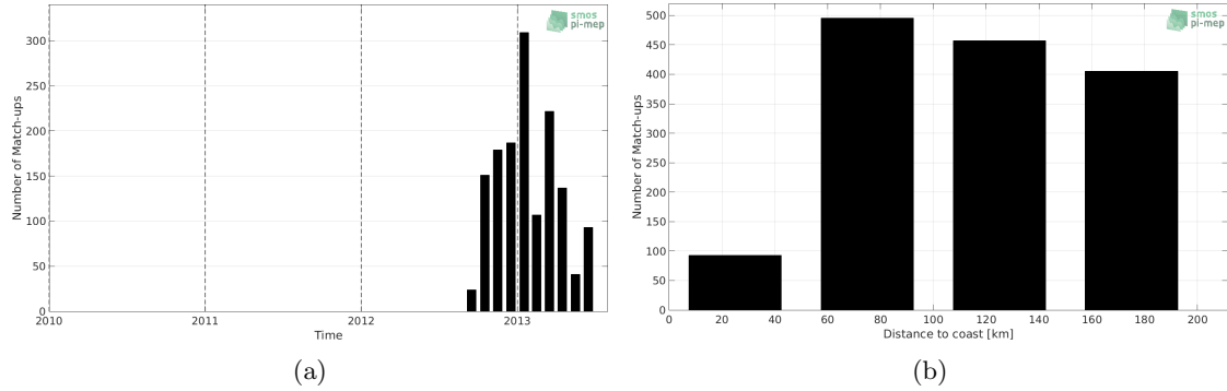
Figure 1: Number of match-ups between Surface drifters and Aquarius-L2-OR-V5 SSS as a function of time (a) and as function of the distance to coast (b) over the Mediterranean Sea Pi-MEP region and for the full satellite product period.
