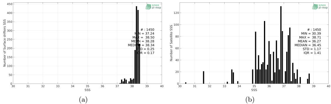
Figure 2: Histograms of SSS from Surface drifters (a) and Aquarius-L2-OR-V5 (b) considering all match-up pairs per bins of 0.1 over the Mediterranean Sea Pi-MEP region and for the full satellite product period.
