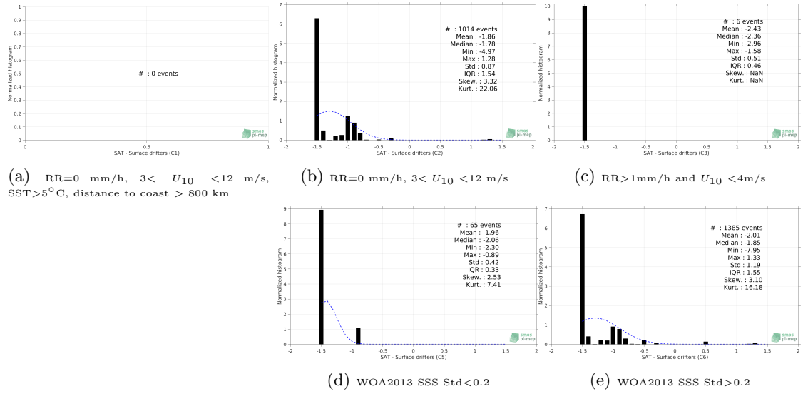
Figure 12: Normalized histogram of \Delta SSS (Aquarius-L2-OR-V5 - Surface drifters) for 5 different subdatasets corresponding to: RR=0 mm/h, 3 < U_{10} < 12 m/s, SST > 5°C, distance to coast > 800 km (a), RR=0 mm/h, 3 < U_{10} < 12 m/s (b), RR > 1mm/h and U_{10} < 4 m/s (c), WOA2013 SSS Std < 0.2 (d), WOA2013 SSS Std > 0.2 (e).
