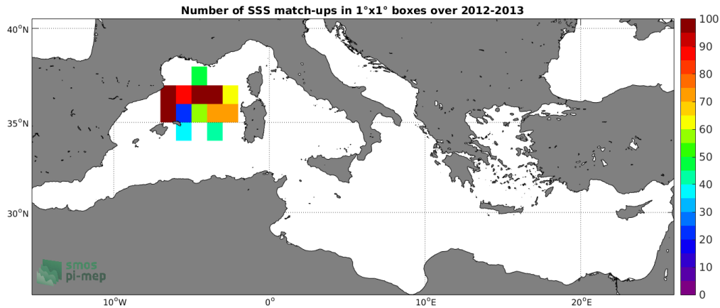
Figure 3: Number of SSS match-ups between Surface drifters SSS and the Aquarius-L2-OR-V5 SSS product for the Mediterranean Sea Pi-MEP region over 1^\circ \times 1^\circ boxes and for the full satellite product period.
