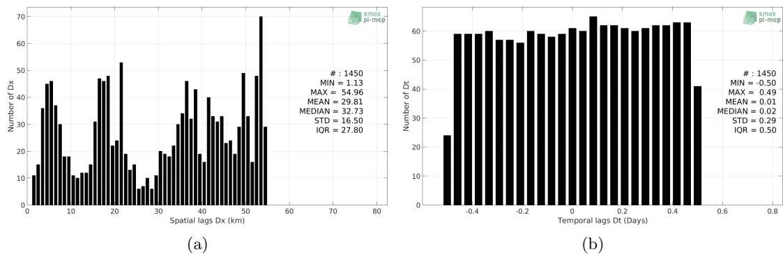
Figure 4: Histograms of the spatial (a) and temporal (b) lags between the time of the Surface drifters measurements and the date of the corresponding Aquarius-L2-OR-V5 SSS product.
