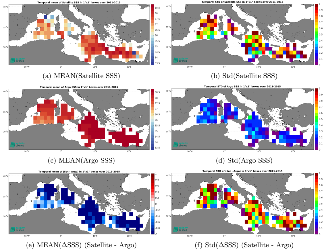
Figure 7: Temporal mean (left) and Std (right) of SSS from Aquarius SSS L2 OR v5 (NASA-GSFC) (top), Argo (middle), and of \Delta\text{SSS} (Satellite - Argo). Only match-up pairs are used to generate these maps.
