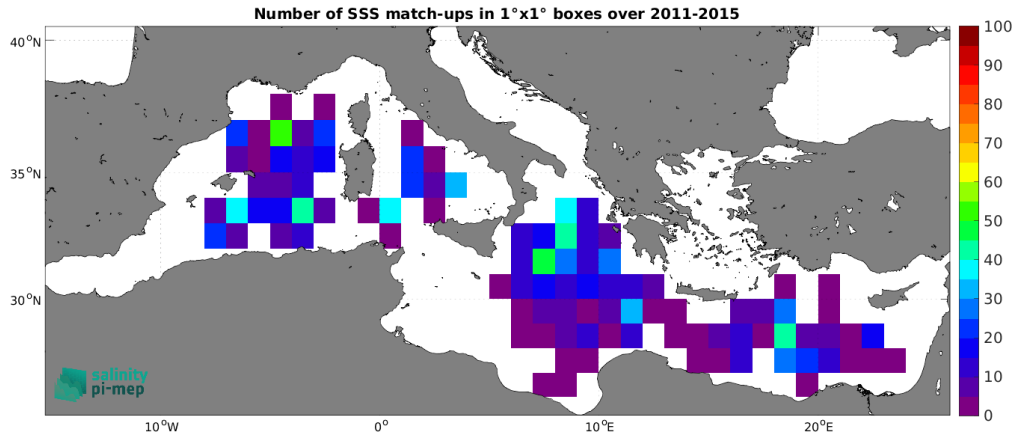
Figure 5: Number of SSS match-ups between Argo SSS and the Aquarius SSS L2 OR v5 (NASA-GSFC) SSS product for the Mediterranean Sea Pi-MEP region over 1^\circ \times 1^\circ boxes and for the full satellite product period.
