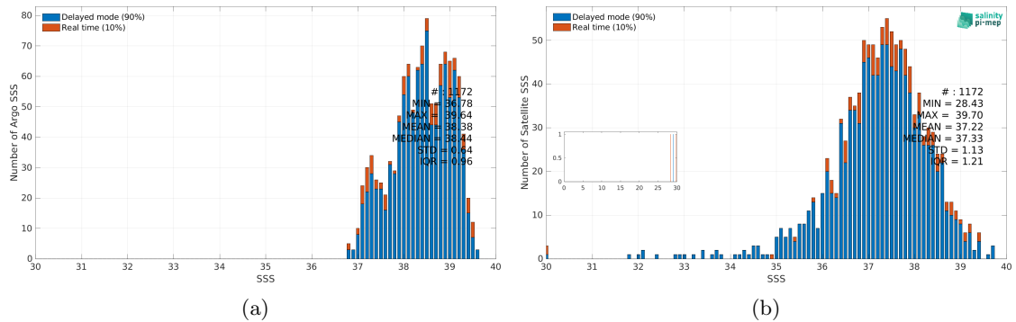
Figure 3: Histograms of SSS from Argo (a) and Aquarius SSS L2 OR v5 (NASA-GSFC) (b) considering all match-up pairs per bins of 0.1 over the Mediterranean Sea Pi-MEP region and for the full satellite product period.
