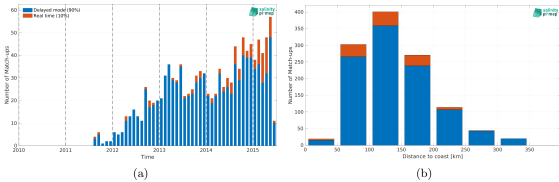
Figure 2: Number of match-ups between Argo and Aquarius SSS L2 OR v5 (NASA-GSFC) SSS as a function of time (a) and as function of the distance to coast (b) over the Mediterranean Sea Pi-MEP region and for the full satellite product period.
