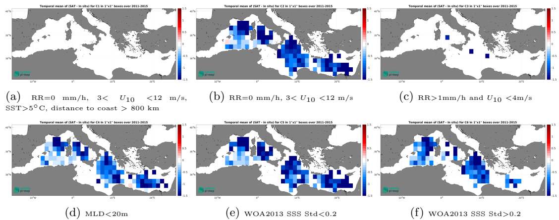
Figure 14: Temporal mean gridded over spatial boxes of size 1^\circ \times 1^\circ of \Delta SSS (Aquarius SSS L2 OR v5 (NASA-GSFC) - Argo) for 6 different subdatasets corresponding to:RR=0 mm/h, 3 < U_{10} < 12 m/s, SST>5°C, distance to coast > 800 km (a), RR=0 mm/h, 3 < U_{10} < 12 m/s (b), RR>1mm/h and U_{10} < 4 m/s (c),MLD<20m (d),WOA2013 SSS Std<0.2 (e),WOA2013 SSS Std>0.2 (f).
