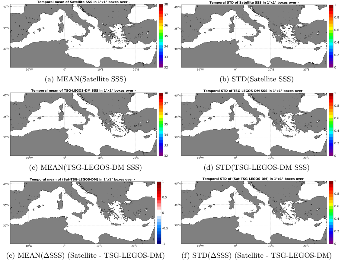
Figure 6: Temporal mean (left) and STD (right) of SSS from AQUARIUS-L2-JPL-V4 (top), TSG-LEGOS-DM (middle), and of \Delta\text{SSS} (Satellite - TSG-LEGOS-DM). Only match-up pairs are used to generate these maps.
