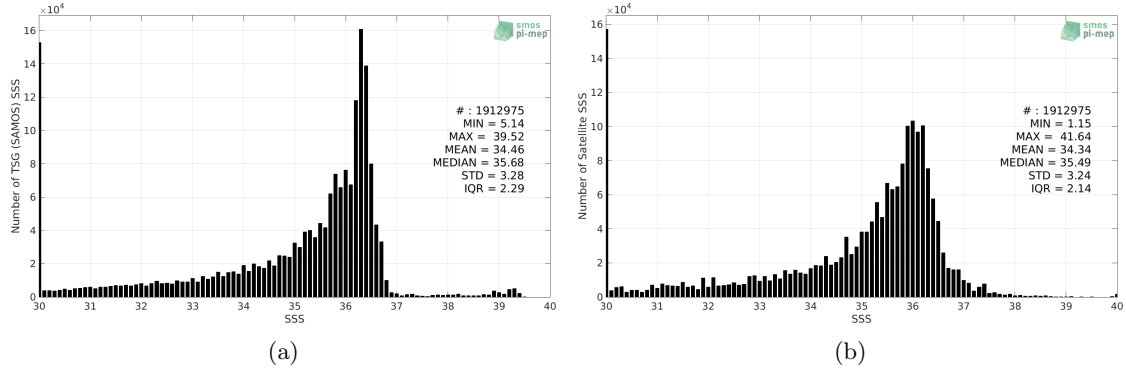
Figure 2: Histograms of SSS from TSG (SAMOS) (a) and SMOS and SMAP SSS L4 OI v1 - 7 Days (LOPS) (b) considering all match-up pairs per bins of 0.1 over the Mississippi river plume Pi-MEP region and for the full satellite product period.
