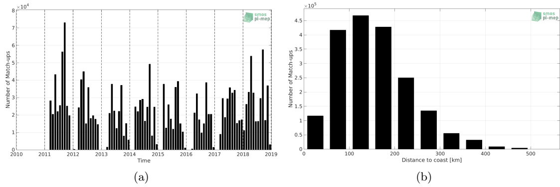
Figure 1: Number of match-ups between TSG (SAMOS) and SMOS and SMAP SSS L4 OI v1 - 7 Days (LOPS) SSS as a function of time (a) and as function of the distance to coast (b) over the Mississippi river plume Pi-MEP region and for the full satellite product period.
