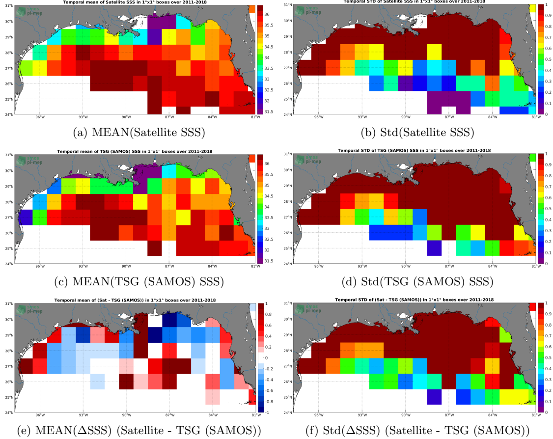
Figure 6: Temporal mean (left) and Std (right) of SSS from SMOS and SMAP SSS L4 OI v1 - 7 Days (LOPS) (top), TSG (SAMOS) (middle), and of \Delta\text{SSS} (Satellite - TSG (SAMOS)). Only match-up pairs are used to generate these maps.
