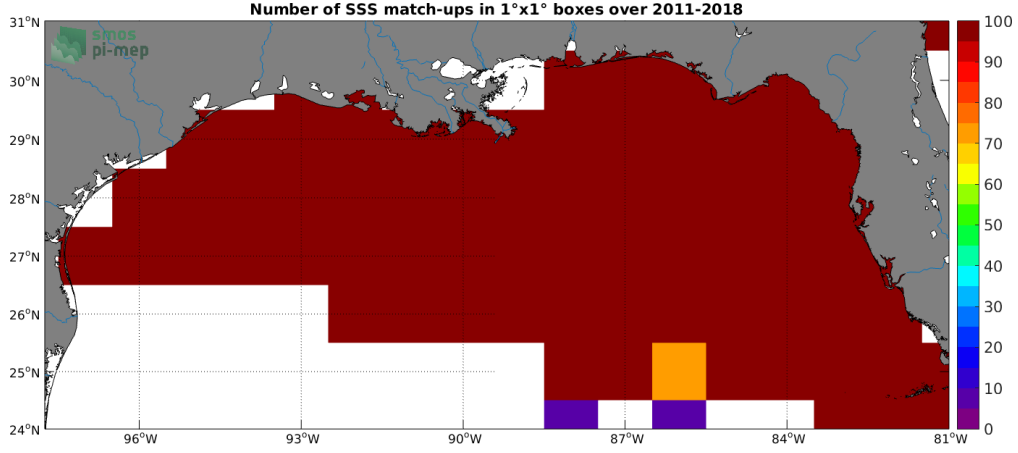
Figure 4: Number of SSS match-ups between TSG (SAMOS) SSS and the SMOS and SMAP SSS L4 OI v1 - 7 Days (LOPS) SSS product for the Mississippi river plume Pi-MEP region over 1^\circ \times 1^\circ boxes and for the full satellite product period.
