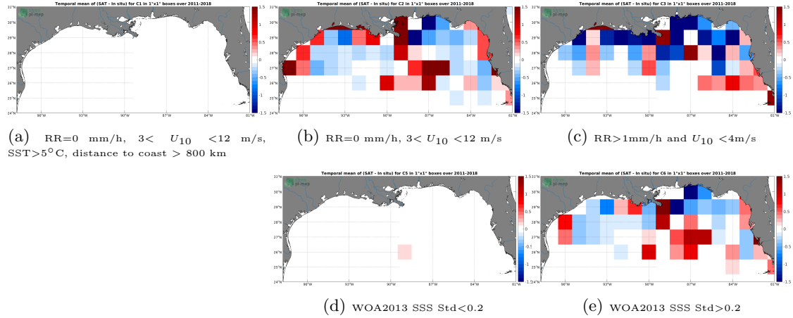
Figure 12: Temporal mean gridded over spatial boxes of size 1^{\circ}\times 1^{\circ} of \Delta\text{SSS} (SMOS and SMAP SSS L4 OI v1 - 7 Days (LOPS) - TSG (SAMOS)) for 5 different subdatasets corresponding to: RR=0 mm/h, 3 < U_{10} < 12 m/s, SST >5^{\circ}\text{C} , distance to coast > 800 km (a), RR=0 mm/h, 3 < U_{10} < 12 m/s (b), RR >1 mm/h and U_{10} < 4 m/s (c), WOA2013 SSS Std <0.2 (d), WOA2013 SSS Std >0.2 (e).
