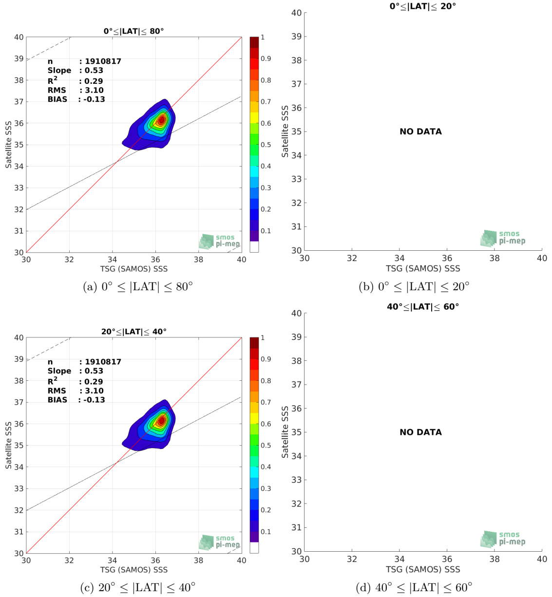
Figure 9: Contour maps of the concentration of SMOS and SMAP SSS L4 OI v1 - 7 Days (LOPS) SSS (y-axis) versus TSG (SAMOS) SSS (x-axis) at match-up pairs for different latitude bands. For each plot, the red line shows x=y . The black thin and dashed lines indicate a linear fit through the data cloud and the \pm 95\% confidence levels, respectively. The number match-up pairs n , the slope and R^2 coefficient of the linear fit, the root mean square (RMS) and the mean bias between satellite and in situ data are indicated for each latitude band in each plots.
