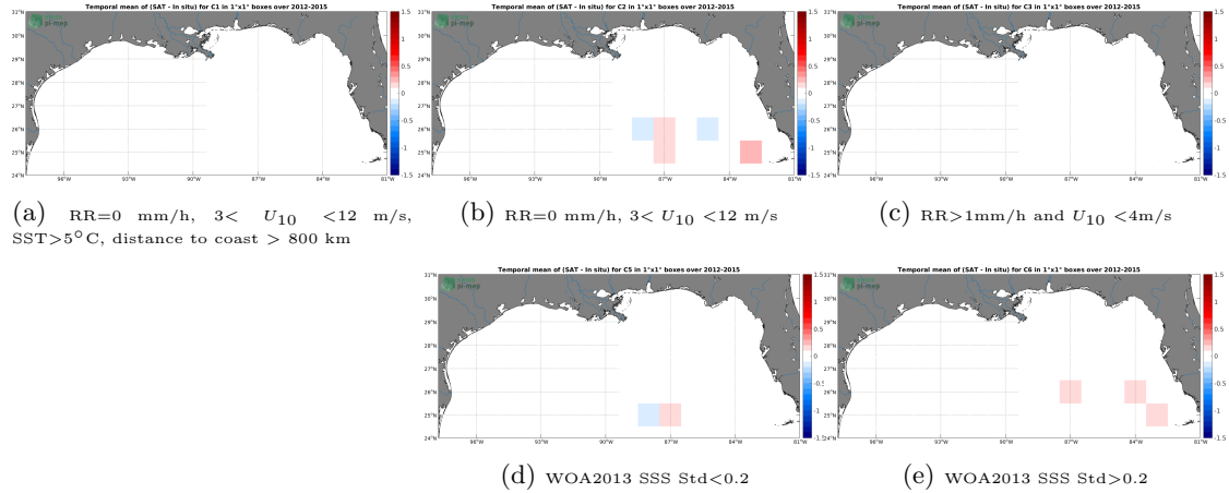
Figure 12: Temporal mean gridded over spatial boxes of size 1^\circ \times 1^\circ of \Delta SSS (SMOS and SMAP SSS L4 OI v1 - 7 Days (LOPS) - TSG (GOSUD-Sailing-ship)) for 5 different subdatasets corresponding to: RR=0 mm/h, 3 < U_{10} < 12 m/s, SST >5^\circ\text{C} , distance to coast > 800 km (a), RR=0 mm/h, 3 < U_{10} < 12 m/s (b), RR >1 mm/h and U_{10} < 4 m/s (c), WOA2013 SSS Std <0.2 (d), WOA2013 SSS Std >0.2 (e).
