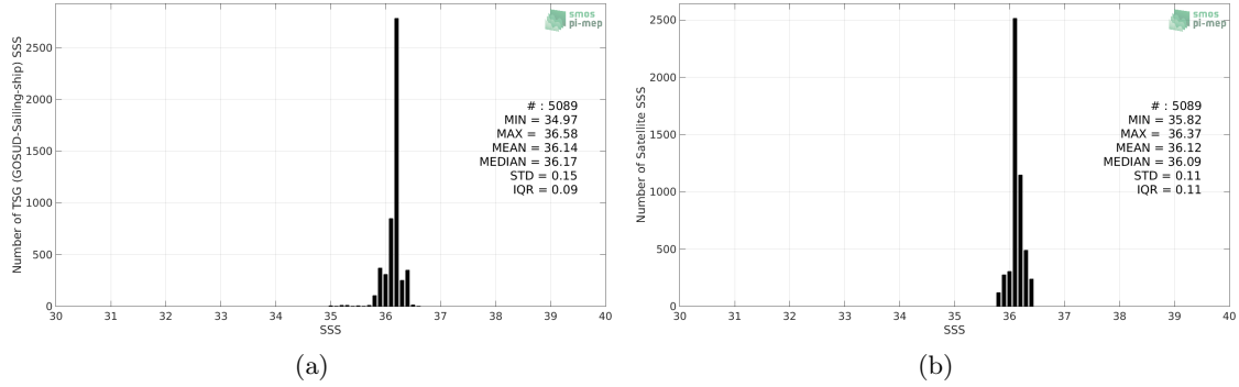
Figure 2: Histograms of SSS from TSG (GOSUD-Sailing-ship) (a) and SMOS and SMAP SSS L4 OI v1 - 7 Days (LOPS) (b) considering all match-up pairs per bins of 0.1 over the Mississippi river plume Pi-MEP region and for the full satellite product period.
