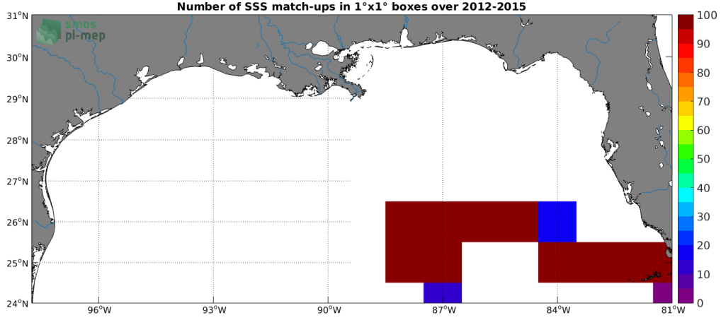
Figure 4: Number of SSS match-ups between TSG (GOSUD-Sailing-ship) SSS and the SMOS and SMAP SSS L4 OI v1 - 7 Days (LOPS) SSS product for the Mississippi river plume Pi-MEP region over 1^\circ \times 1^\circ boxes and for the full satellite product period.
