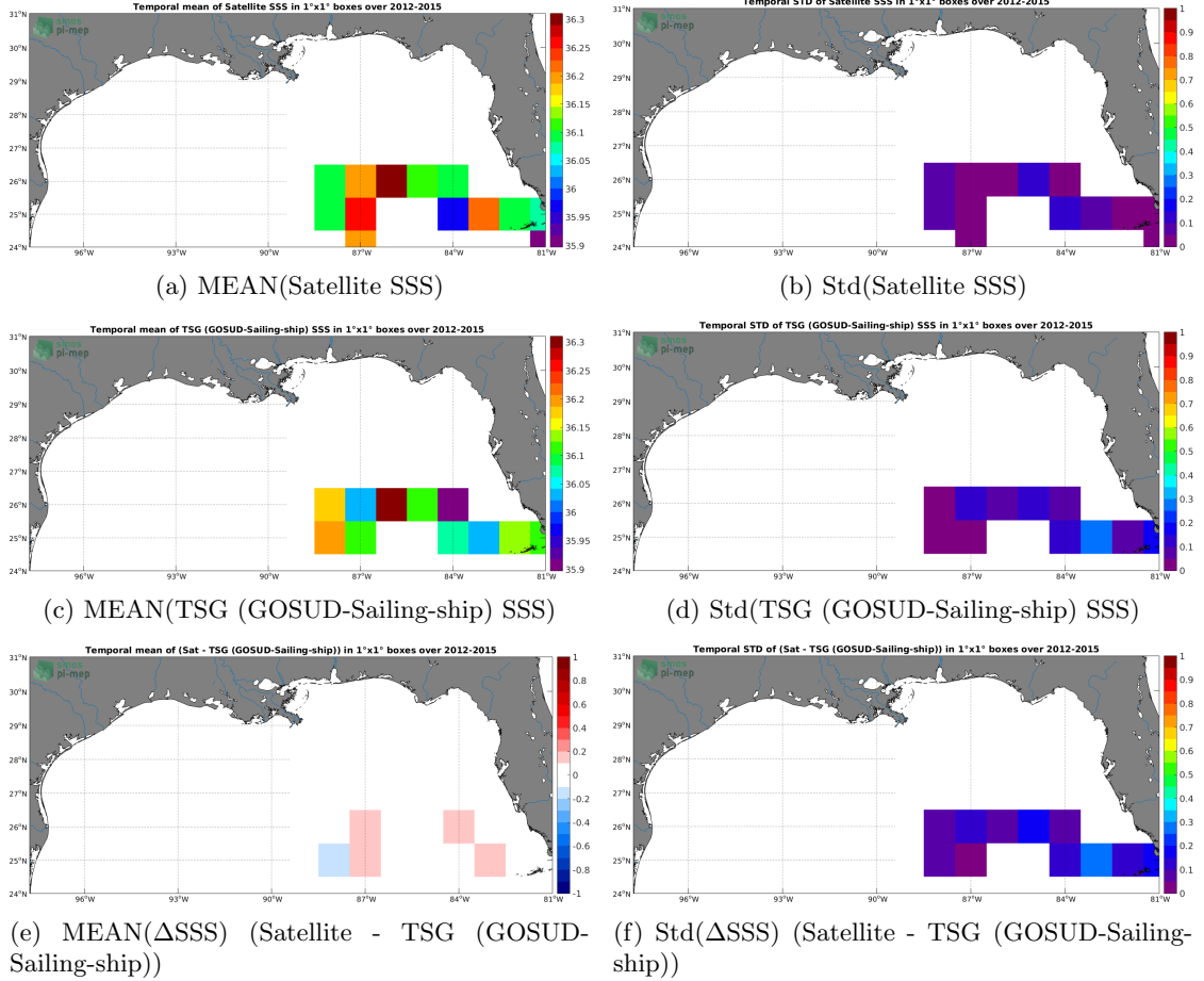
Figure 6: Temporal mean (left) and Std (right) of SSS from SMOS and SMAP SSS L4 OI v1 - 7 Days (LOPS) (top), TSG (GOSUD-Sailing-ship) (middle), and of \Delta\text{SSS} (Satellite - TSG (GOSUD-Sailing-ship)). Only match-up pairs are used to generate these maps.
