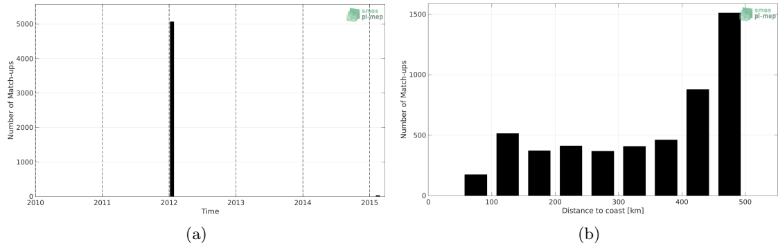
Figure 1: Number of match-ups between TSG (GOSUD-Sailing-ship) and SMOS and SMAP SSS L4 OI v1 - 7 Days (LOPS) SSS as a function of time (a) and as function of the distance to coast (b) over the Mississippi river plume Pi-MEP region and for the full satellite product period.
