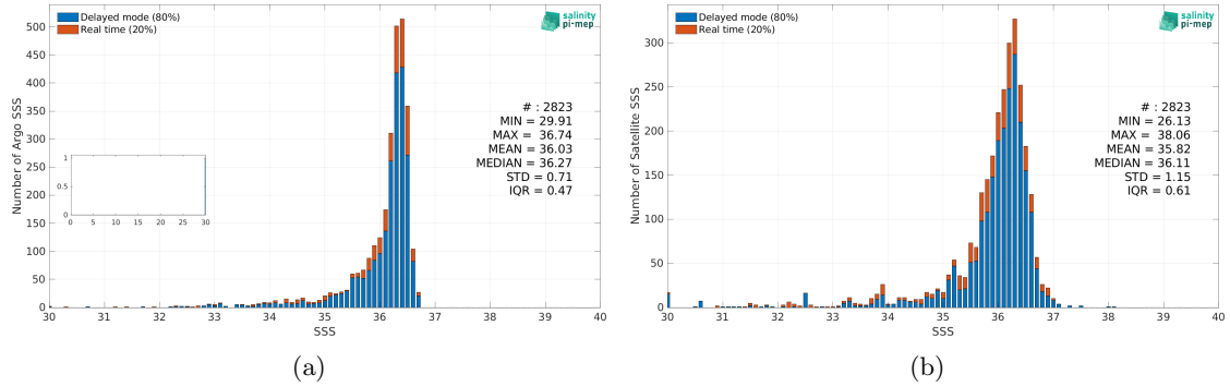
Figure 2: Histograms of SSS from Argo (a) and SMOS and SMAP SSS L4 OI v1 - 7 Days (LOPS) (b) considering all match-up pairs per bins of 0.1 over the Mississippi river plume Pi-MEP region and for the full satellite product period.
