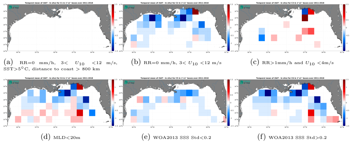
Figure 12: Temporal mean gridded over spatial boxes of size 1^{\circ}\times 1^{\circ} of \Delta\text{SSS} (SMOS and SMAP SSS L4 OI v1 - 7 Days (LOPS) - Argo) for 6 different subdatasets corresponding to:RR=0 mm/h, 3 < U_{10} < 12 m/s, SST > 5^{\circ}\text{C} , distance to coast > 800 km (a), RR=0 mm/h, 3 < U_{10} < 12 m/s (b), RR > 1\text{mm/h} and U_{10} < 4\text{m/s} (c),MLD < 20\text{m} (d),WOA2013 SSS Std < 0.2 (e),WOA2013 SSS Std > 0.2 (f).
