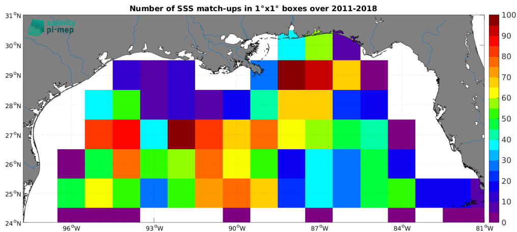
Figure 4: Number of SSS match-ups between Argo SSS and the SMOS and SMAP SSS L4 OI v1 - 7 Days (LOPS) SSS product for the Mississippi river plume Pi-MEP region over 1^\circ \times 1^\circ boxes and for the full satellite product period.
