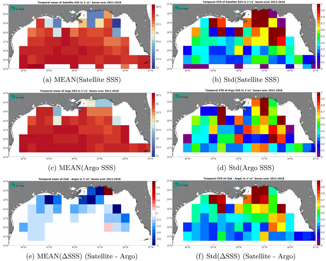
Figure 6: Temporal mean (left) and Std (right) of SSS from SMOS and SMAP SSS L4 OI v1 - 7 Days (LOPS) (top), Argo (middle), and of \Delta\text{SSS} (Satellite - Argo). Only match-up pairs are used to generate these maps.
