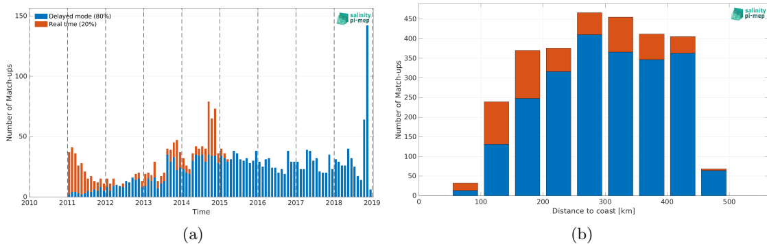
Figure 1: Number of match-ups between Argo and SMOS and SMAP SSS L4 OI v1 - 7 Days (LOPS) SSS as a function of time (a) and as function of the distance to coast (b) over the Mississippi river plume Pi-MEP region and for the full satellite product period.
