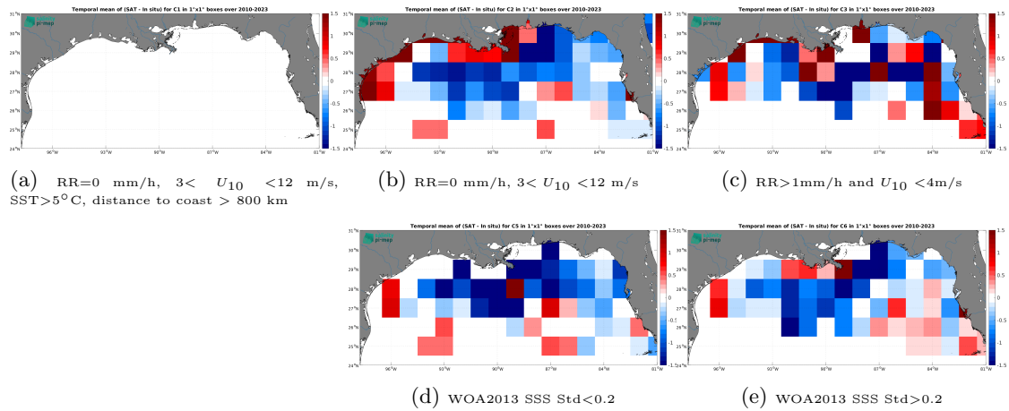
Figure 12: Temporal mean gridded over spatial boxes of size 1^{\circ}\times 1^{\circ} of \Delta\text{SSS} (SMOS SSS L4 v1 - Weekly (CMEMS-CNR) - TSG (SAMOS)) for 5 different subdatasets corresponding to:RR=0 mm/h, 3 < U_{10} < 12 m/s, SST >5^{\circ}\text{C} , distance to coast > 800 km (a), RR=0 mm/h, 3 < U_{10} < 12 m/s (b), RR >1 mm/h and U_{10} < 4 m/s (c), WOA2013 SSS Std <0.2 (d), WOA2013 SSS Std >0.2 (e).
