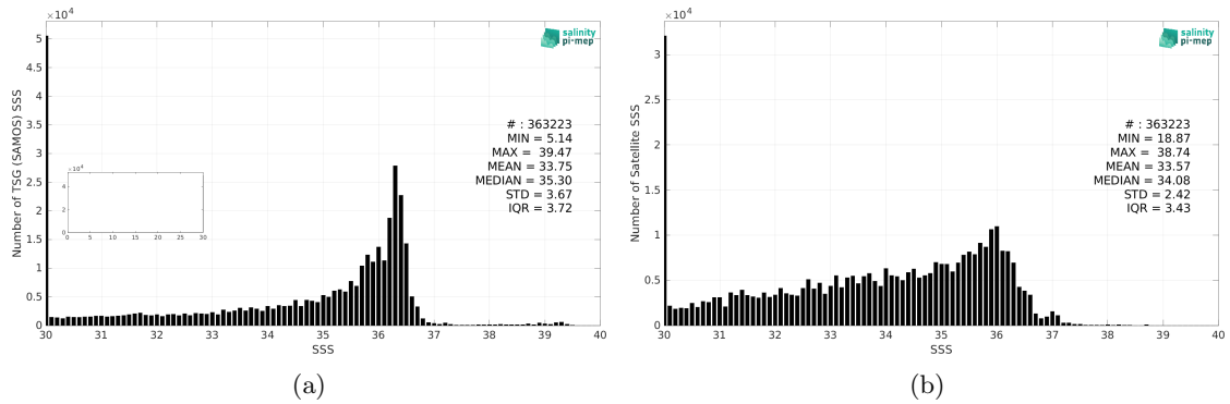
Figure 2: Histograms of SSS from TSG (SAMOS) (a) and SMOS SSS L4 v1 - Weekly (CMEMS-CNR) (b) considering all match-up pairs per bins of 0.1 over the Mississippi river plume Pi-MEP region and for the full satellite product period.
