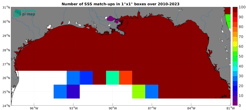
Figure 4: Number of SSS match-ups between TSG (SAMOS) SSS and the SMOS SSS L4 v1 - Weekly (CMEMS-CNR) SSS product for the Mississippi river plume Pi-MEP region over 1^\circ \times 1^\circ boxes and for the full satellite product period.
