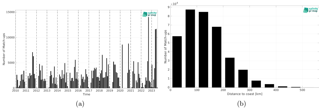
Figure 1: Number of match-ups between TSG (SAMOS) and SMOS SSS L4 v1 - Weekly (CMEMS-CNR) SSS as a function of time (a) and as function of the distance to coast (b) over the Mississippi river plume Pi-MEP region and for the full satellite product period.
