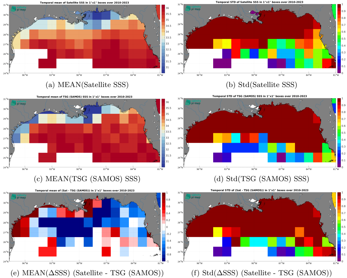
Figure 6: Temporal mean (left) and Std (right) of SSS from SMOS SSS L4 v1 - Weekly (CMEMS-CNR) (top), TSG (SAMOS) (middle), and of \Delta\text{SSS} (Satellite - TSG (SAMOS)). Only match-up pairs are used to generate these maps.
