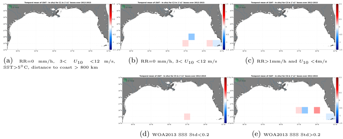
Figure 12: Temporal mean gridded over spatial boxes of size 1^{\circ}\times 1^{\circ} of \Delta SSS (SMOS SSS L4 v1 - Weekly (CMEMS-CNR) - TSG (GOSUD-Sailing-ship)) for 5 different subdatasets corresponding to:RR=0 mm/h, 3 < U_{10} < 12 m/s, SST >5^{\circ}\text{C} , distance to coast > 800 km (a), RR=0 mm/h, 3 < U_{10} < 12 m/s (b), RR >1 mm/h and U_{10} < 4 m/s (c), WOA2013 SSS Std <0.2 (d), WOA2013 SSS Std >0.2 (e).
