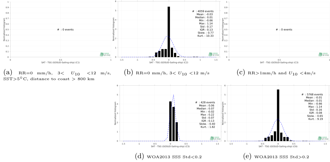
Figure 13: Normalized histogram of \Delta\text{SSS} (SMOS SSS L4 v1 - Weekly (CMEMS-CNR) - TSG (GOSUD-Sailing-ship)) for 5 different subdatasets corresponding to: RR=0 mm/h, 3 < U_{10} < 12 m/s, SST > 5^{\circ}\text{C} , distance to coast > 800 km (a), RR=0 mm/h, 3 < U_{10} < 12 m/s (b), RR > 1\text{mm/h} and U_{10} < 4\text{m/s} (c), WOA2013 SSS Std < 0.2 (d), WOA2013 SSS Std > 0.2 (e).
