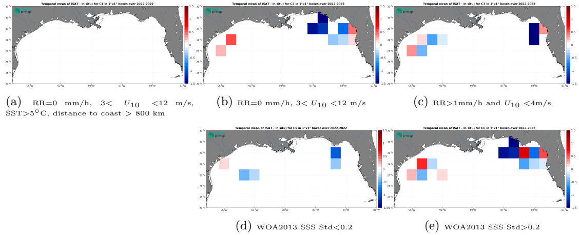
Figure 12: Temporal mean gridded over spatial boxes of size 1^{\circ}\times 1^{\circ} of \Delta\text{SSS} (SMOS SSS L4 v1 - Weekly (CMEMS-CNR) - Saildrone) for 5 different subdatasets corresponding to:RR=0 mm/h, 3 < U_{10} < 12 m/s, SST >5^{\circ}\text{C} , distance to coast > 800 km (a), RR=0 mm/h, 3 < U_{10} < 12 m/s (b), RR >1 mm/h and U_{10} < 4 m/s (c), WOA2013 SSS Std <0.2 (d), WOA2013 SSS Std >0.2 (e).
