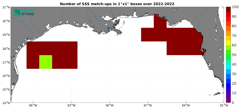
Figure 4: Number of SSS match-ups between Saildrone SSS and the SMOS SSS L4 v1 - Weekly (CMEMS-CNR) SSS product for the Mississippi river plume Pi-MEP region over 1^\circ \times 1^\circ boxes and for the full satellite product period.
