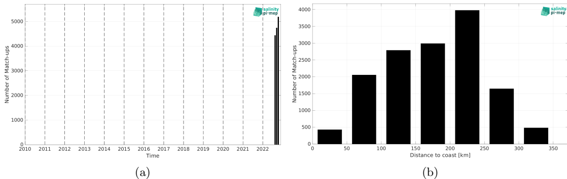
Figure 1: Number of match-ups between Saildrone and SMOS SSS L4 v1 - Weekly (CMEMS-CNR) SSS as a function of time (a) and as function of the distance to coast (b) over the Mississippi river plume Pi-MEP region and for the full satellite product period.
