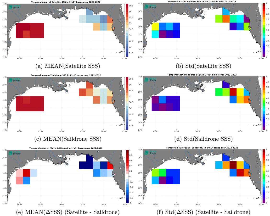
Figure 6: Temporal mean (left) and Std (right) of SSS from SMOS SSS L4 v1 - Weekly (CMEMS-CNR) (top), Saildrone (middle), and of \Delta\text{SSS} (Satellite - Saildrone). Only match-up pairs are used to generate these maps.
