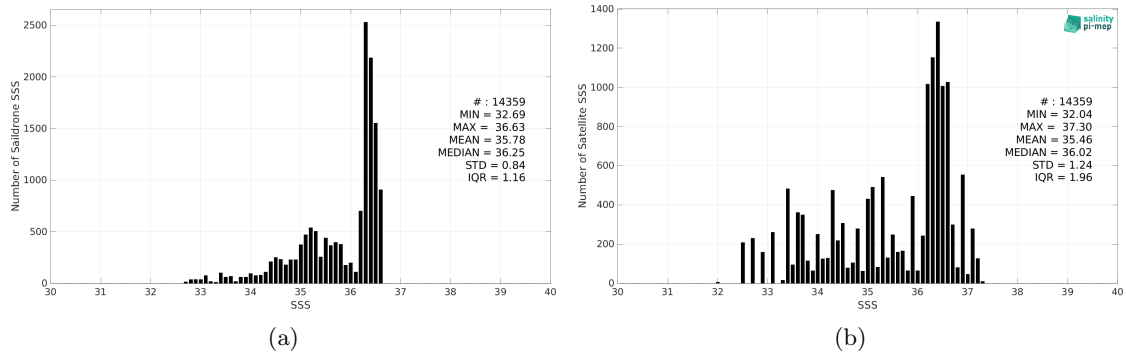
Figure 2: Histograms of SSS from Saildrone (a) and SMOS SSS L4 v1 - Weekly (CMEMS-CNR) (b) considering all match-up pairs per bins of 0.1 over the Mississippi river plume Pi-MEP region and for the full satellite product period.
