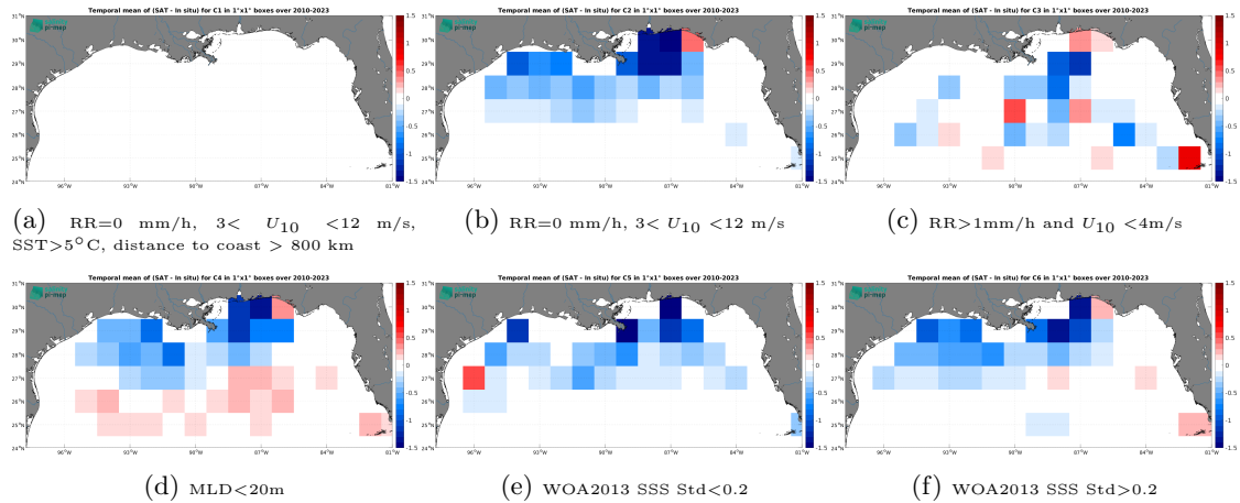
Figure 12: Temporal mean gridded over spatial boxes of size 1^{\circ}\times 1^{\circ} of \Delta\text{SSS} (SMOS SSS L4 v1 - Weekly (CMEMS-CNR) - Argo) for 6 different subdatasets corresponding to:RR=0 mm/h, 3 < U_{10} < 12 m/s, SST > 5^{\circ}\text{C} , distance to coast > 800 km (a), RR=0 mm/h, 3 < U_{10} < 12 m/s (b), RR > 1\text{mm/h} and U_{10} < 4\text{m/s} (c),MLD < 20\text{m} (d),WOA2013 SSS Std < 0.2 (e),WOA2013 SSS Std > 0.2 (f).
