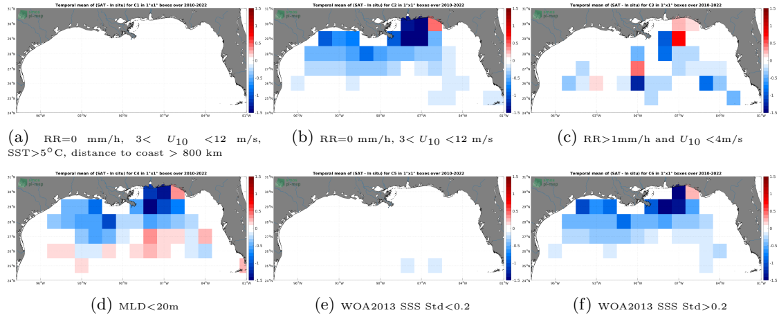
Figure 12: Temporal mean gridded over spatial boxes of size 1^{\circ}\times 1^{\circ} of \Delta\text{SSS} (SMOS SSS L4 v1 - Weekly (CMEMS-CNR) - Argo) for 6 different subdatasets corresponding to: RR=0 mm/h, 3 < U_{10} < 12 m/s, SST > 5^{\circ}\text{C} , distance to coast > 800 km (a), RR=0 mm/h, 3 < U_{10} < 12 m/s (b), RR > 1 mm/h and U_{10} < 4 m/s (c), MLD < 20\text{m} (d), WOA2013 SSS Std < 0.2 (e), WOA2013 SSS Std > 0.2 (f).
