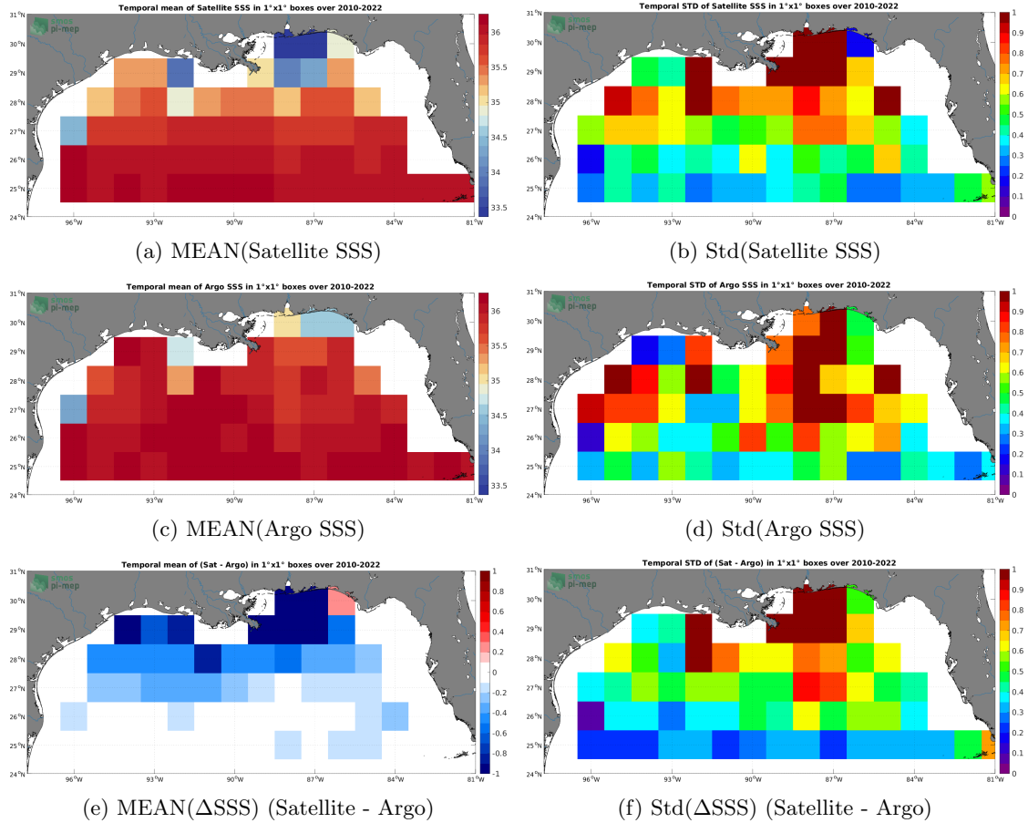
Figure 6: Temporal mean (left) and Std (right) of SSS from SMOS SSS L4 v1 - Weekly (CMEMS-CNR) (top), Argo (middle), and of \Delta\text{SSS} (Satellite - Argo). Only match-up pairs are used to generate these maps.
